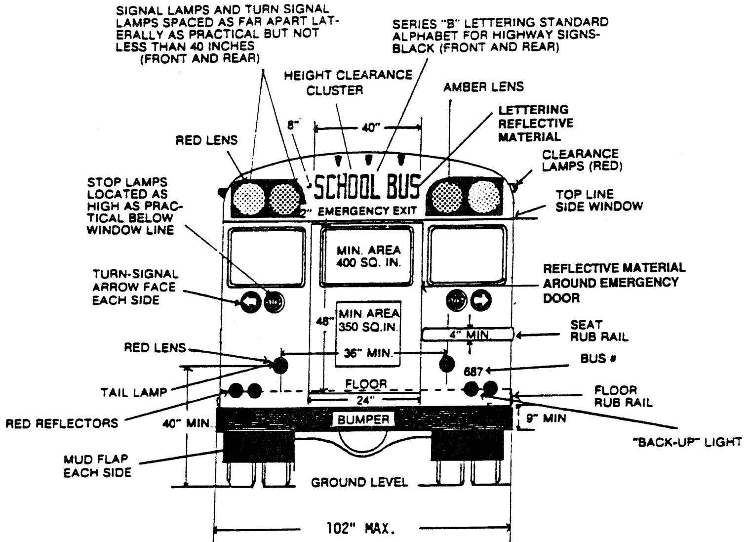
REAR ELEVATION
