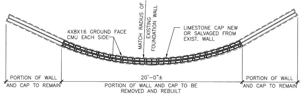
2 PLAN VIEW 1/4"=1'-0"
