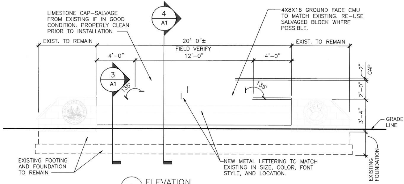
1 ELEVATION 1/4"=1'-0"
