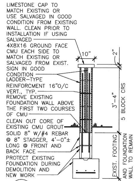
3 SECTION 1/2"=1'-0"
