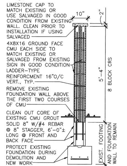
4 SECTION 1/2"=1'-0"
