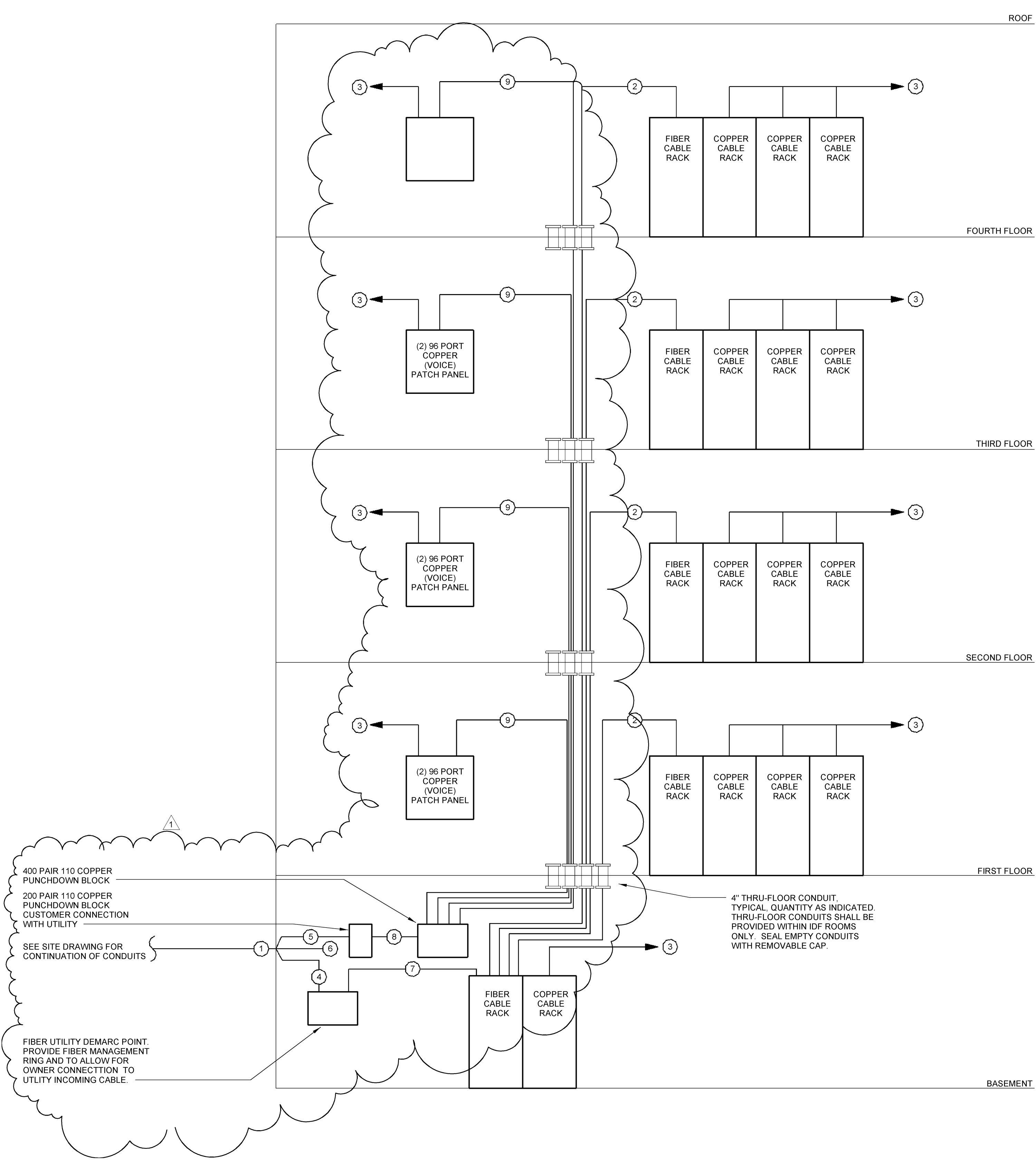
1 TELECOMMUNICATIONS RISER DIAGRAM NOT TO SCALE
