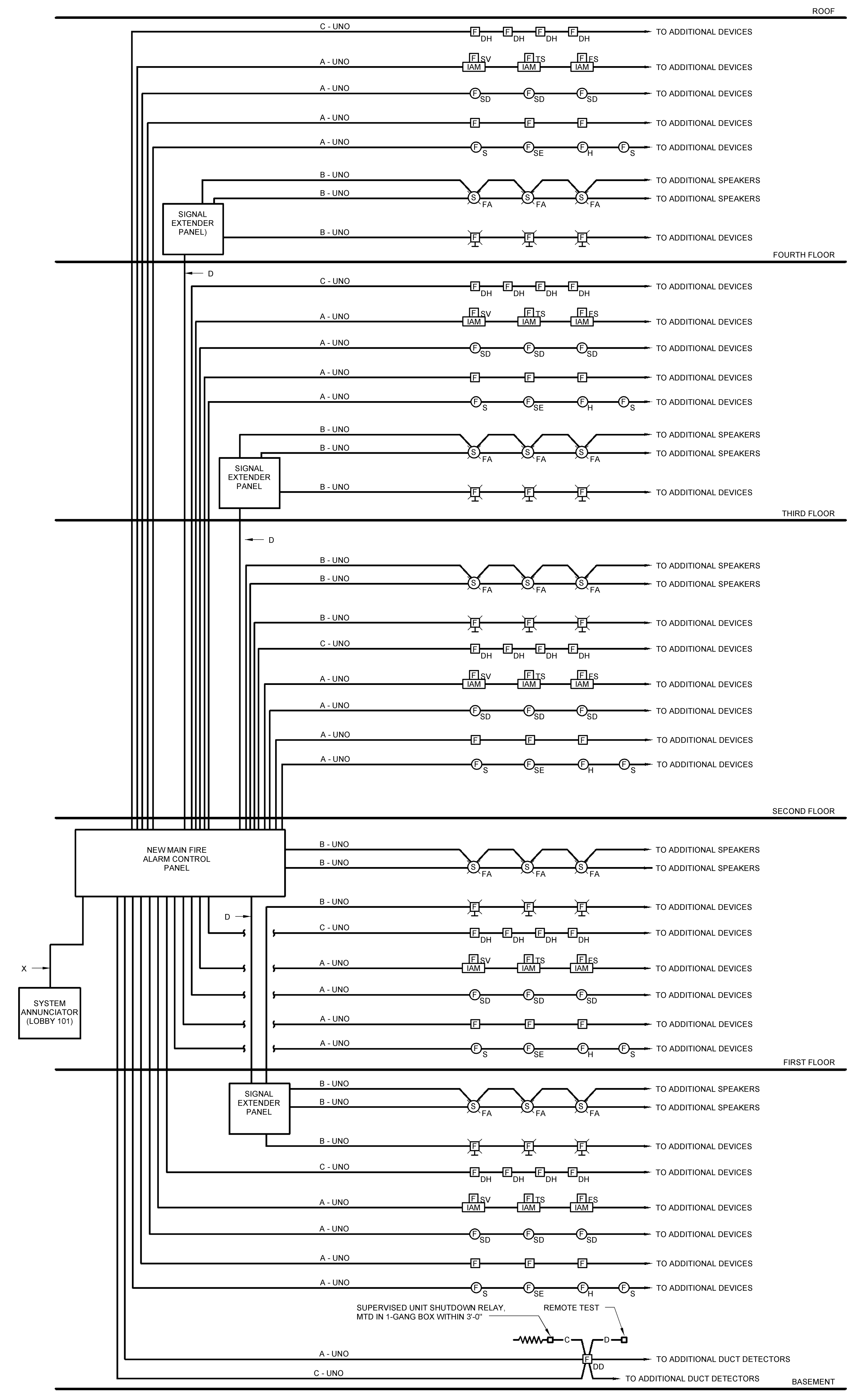
2 FIRE ALARM SYSTEM RISER DIAGRAM NOT TO SCALE
