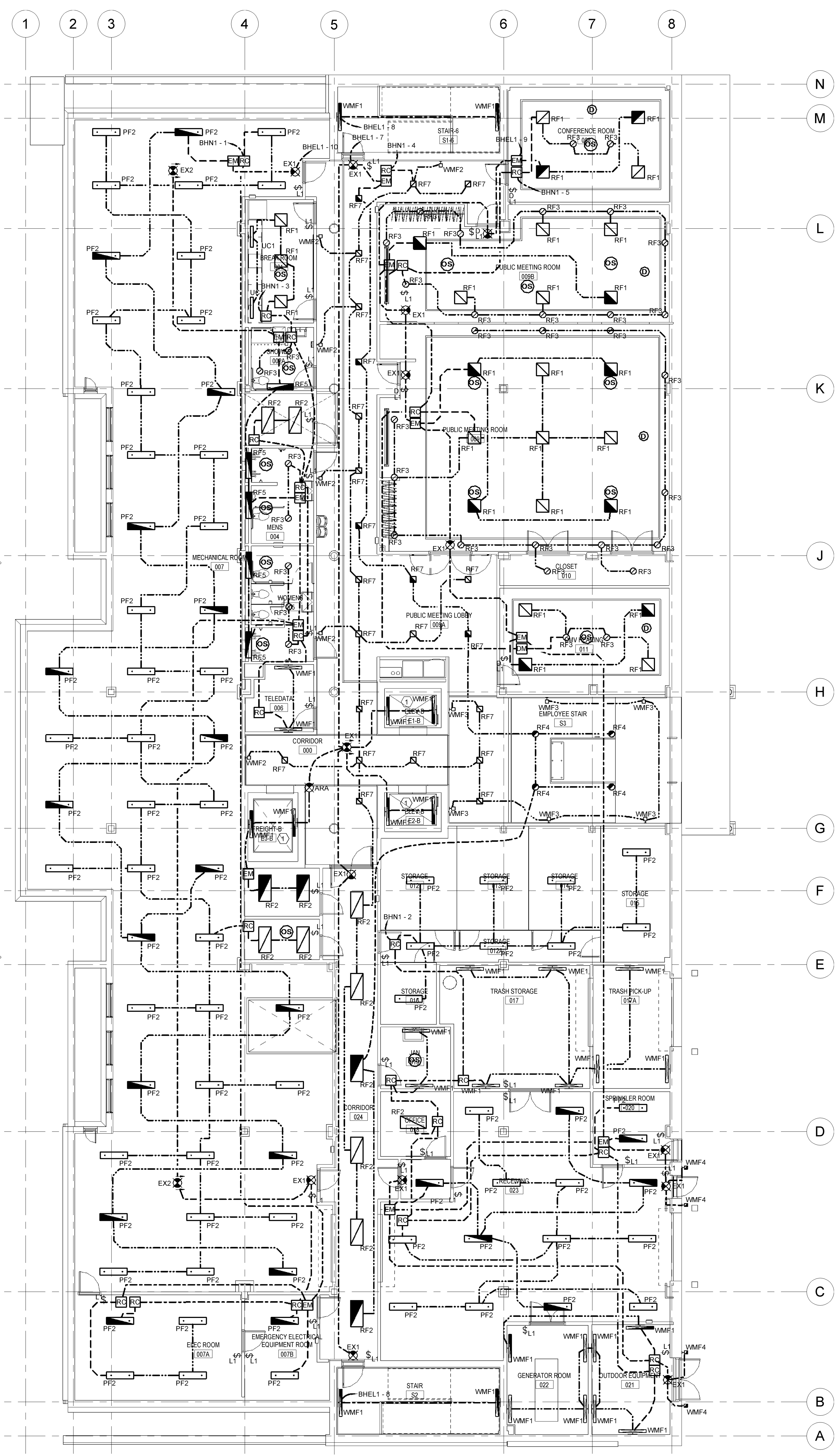
1 ELECTRICAL BASEMENT FLOOR PLAN - LIGHTING SCALE: 1/8" = 1'-0"
