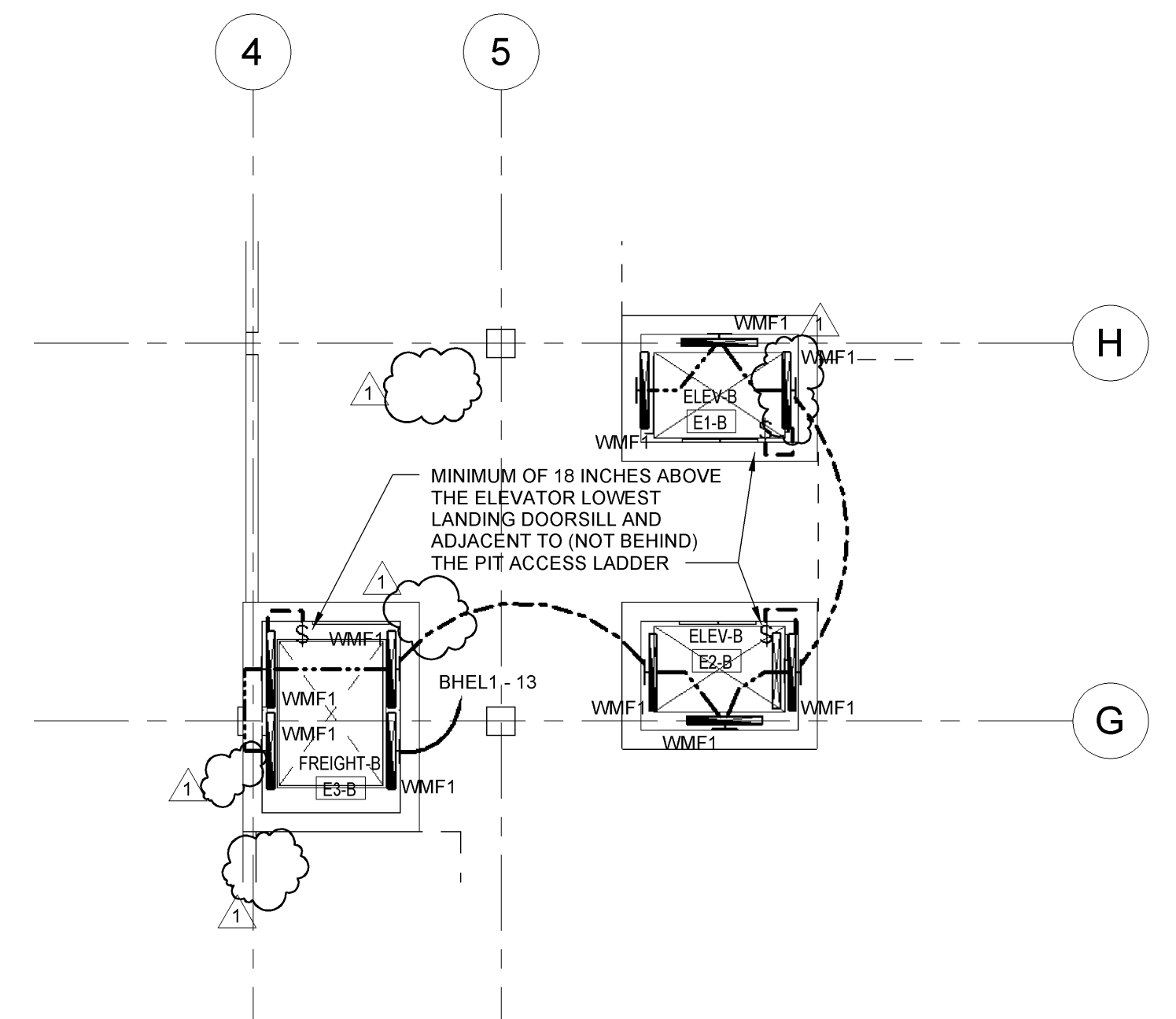
2 ELECTRICAL ELEVATOR PIT PLAN - LIGHTING SCALE: 1/8" = 1'-0"
