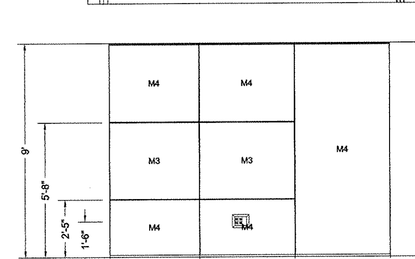
Elevation M
