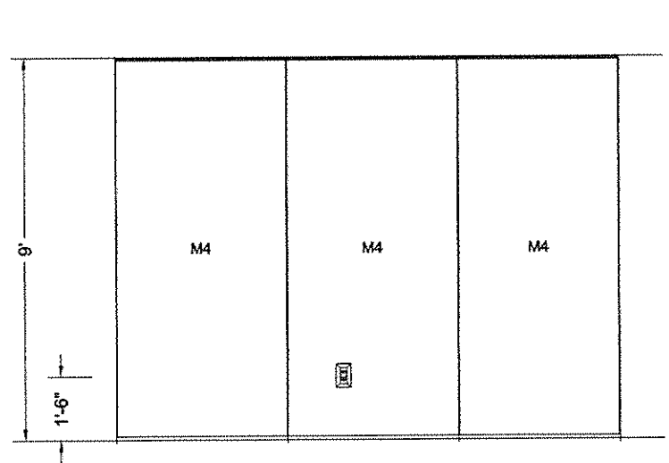
Elevation Q
