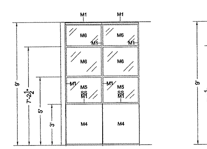
Elevation AA
