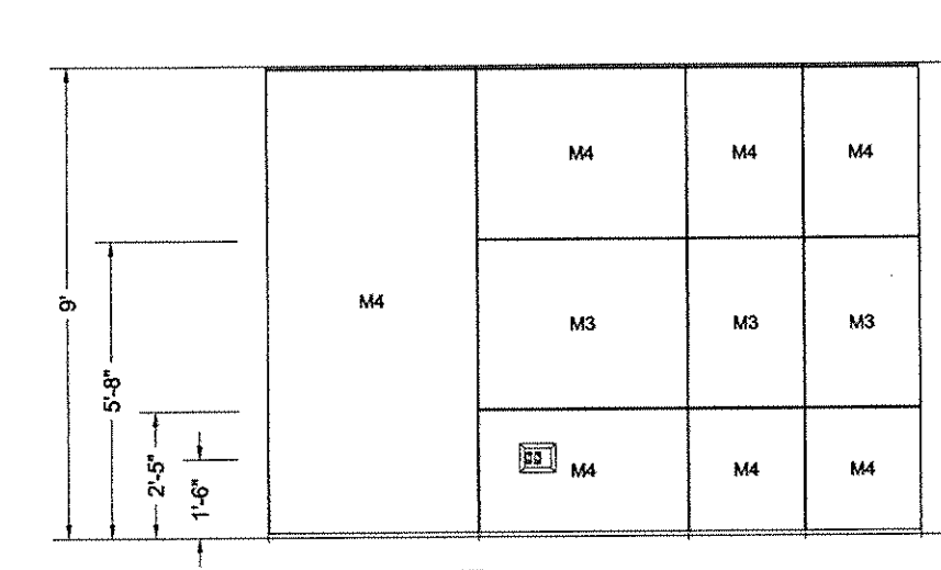
Elevation F
