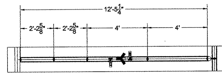
Elevation D
