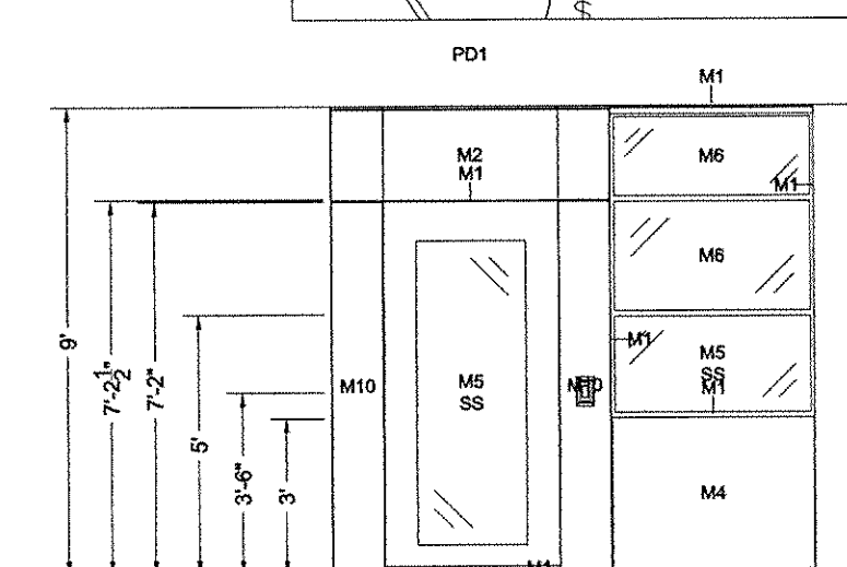
Elevation W
