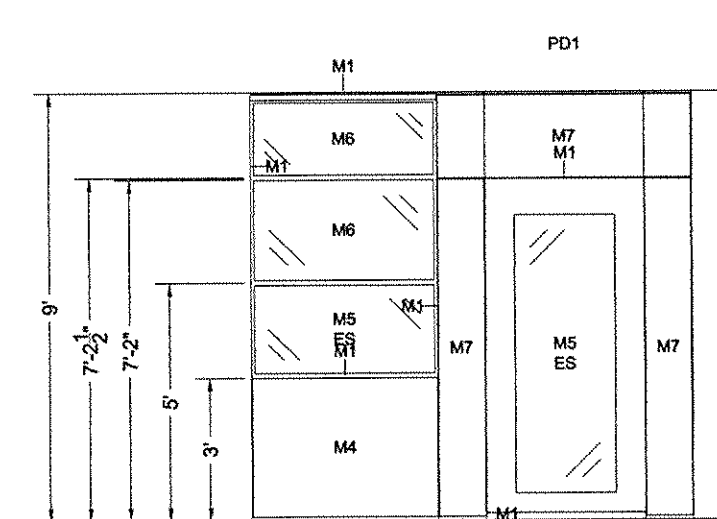
Elevation X
