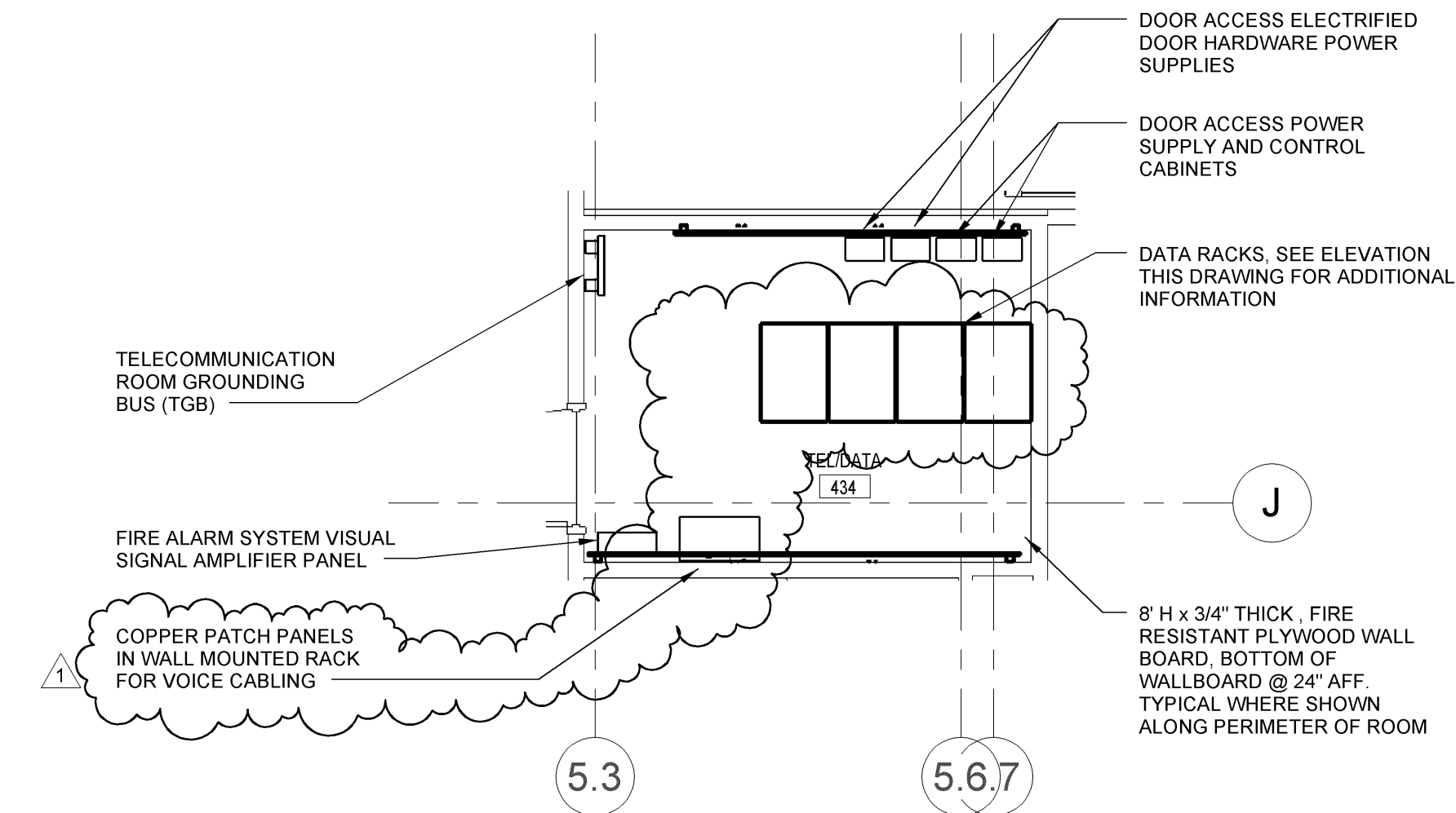
2 ENLARGED TELE/DATA ROOM FLOOR PLAN SCALE: 1/4" = 1'-0"
