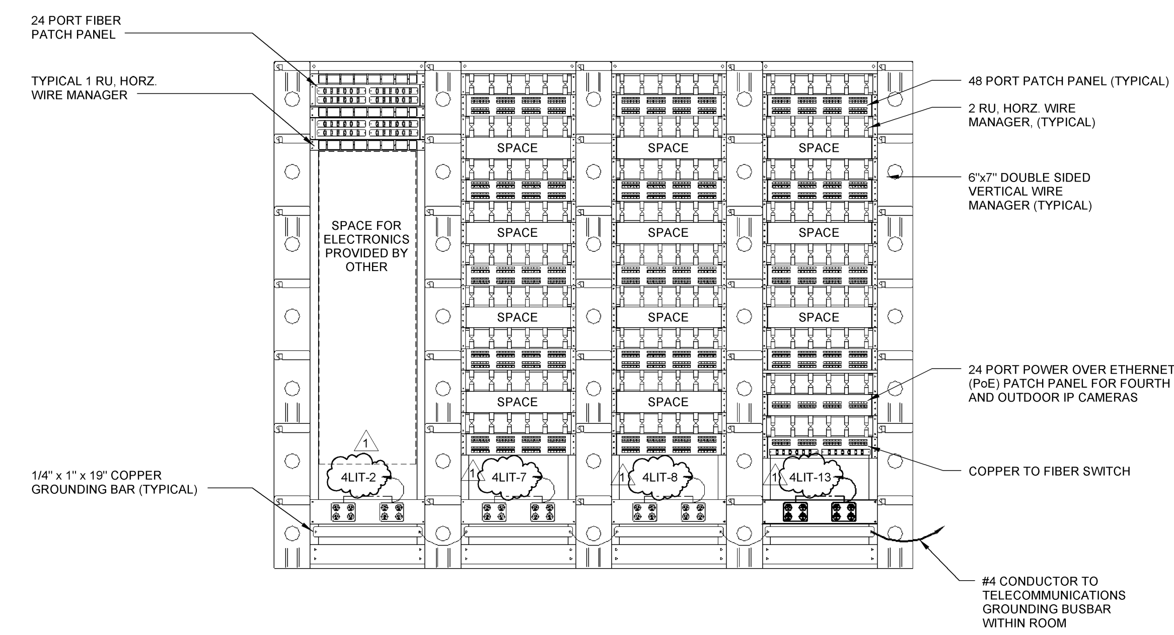
3 FOURTH FLOOR TELECOMMUNICATION RACK ELEVATION NOT TO SCALE
