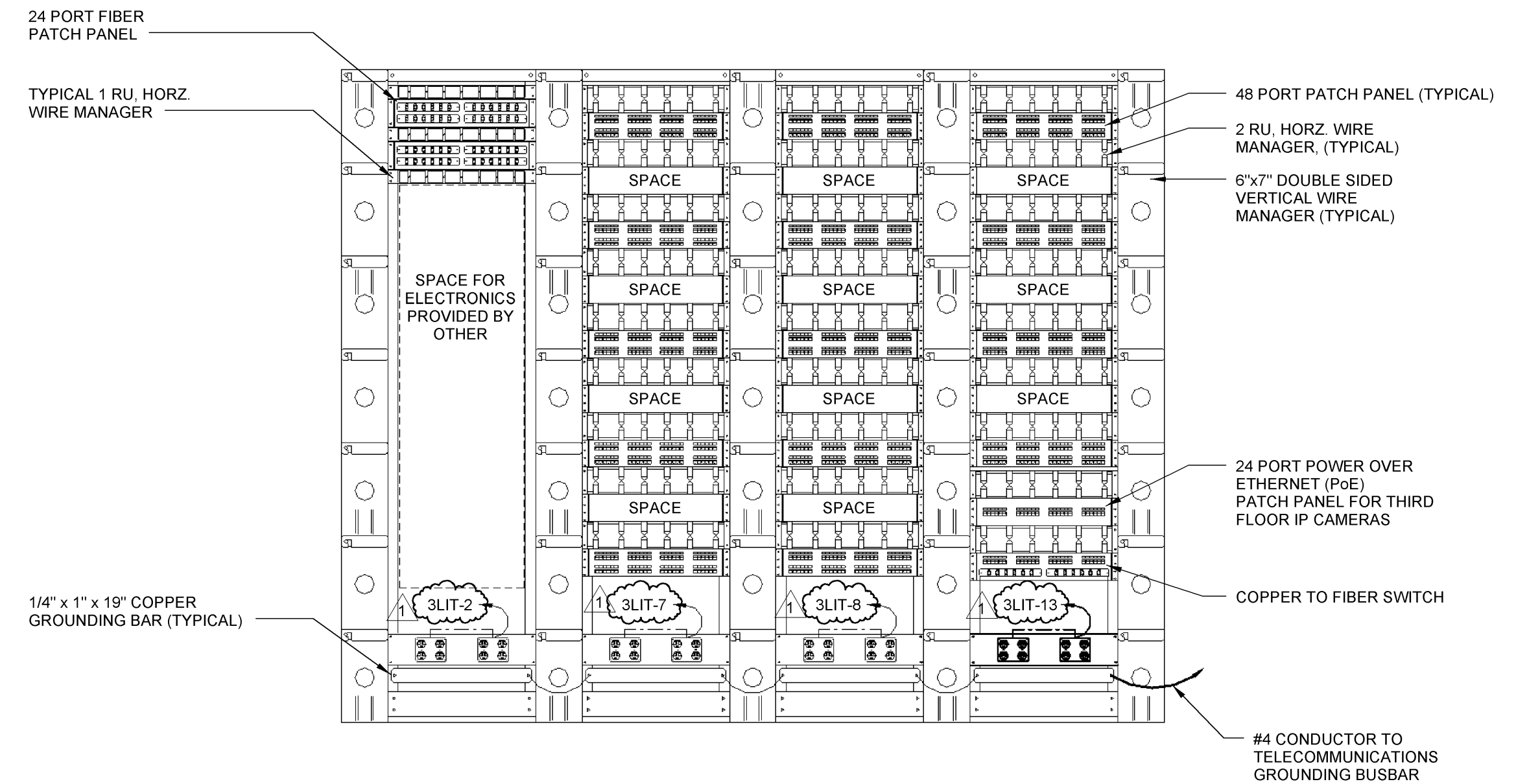
3 THIRD FLOOR TELECOMMUNICATION RACK ELEVATION NOT TO SCALE
