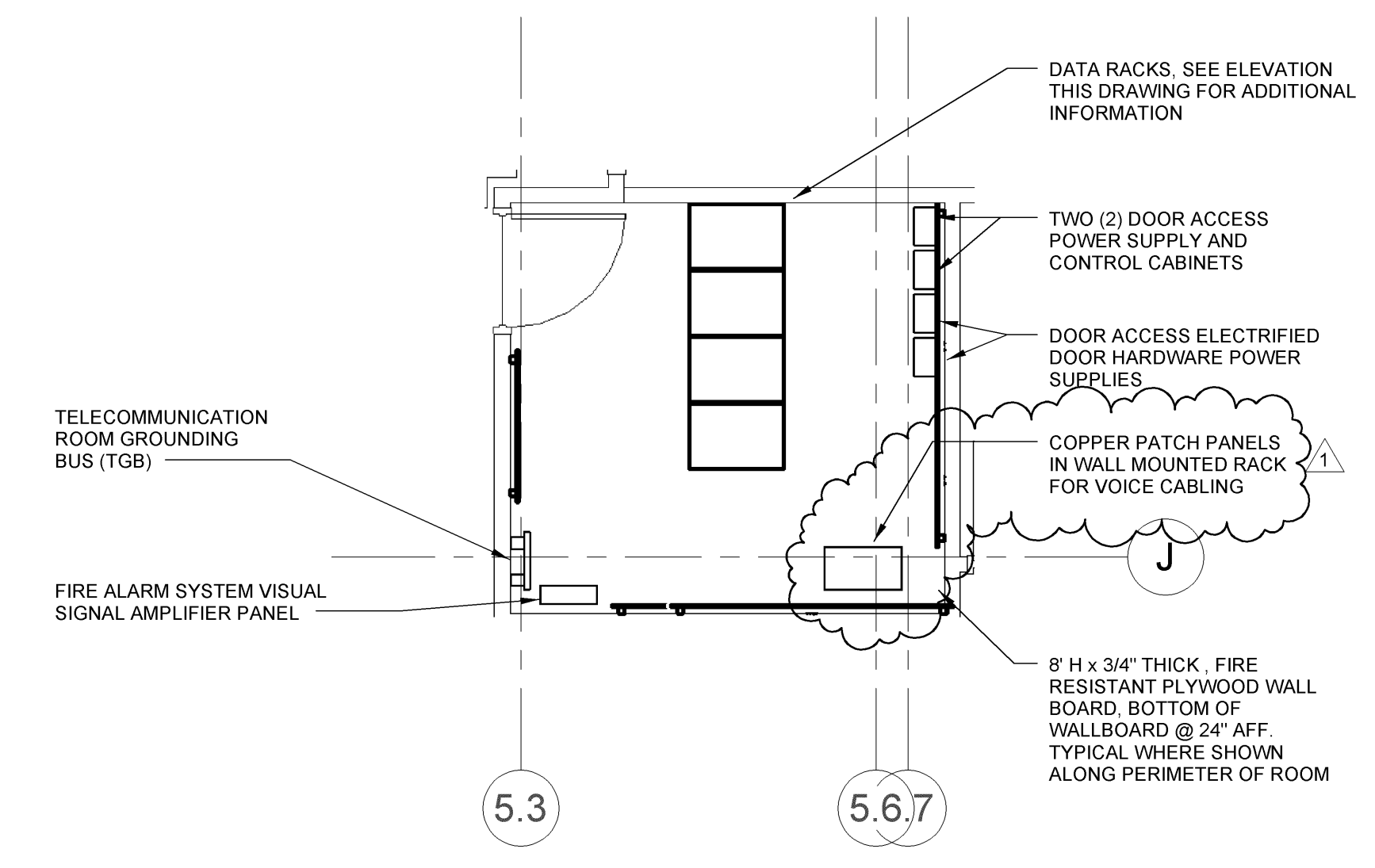
2 Callout of TELEDATA ROOM 302 SCALE: 1/4" = 1'-0"
