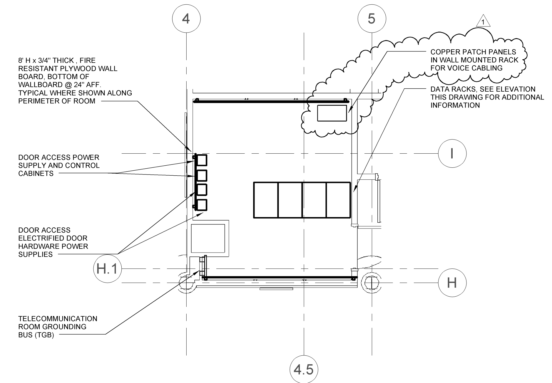
2 ENLARGED TELE/DATA ROOM FLOOR PLAN SCALE: 1/4" = 1'-0"
