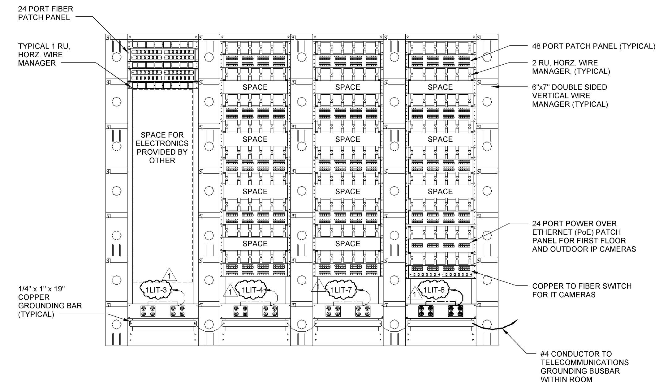
3 FIRST FLOOR TELECOMMUNICATION RACK ELEVATION NOT TO SCALE
