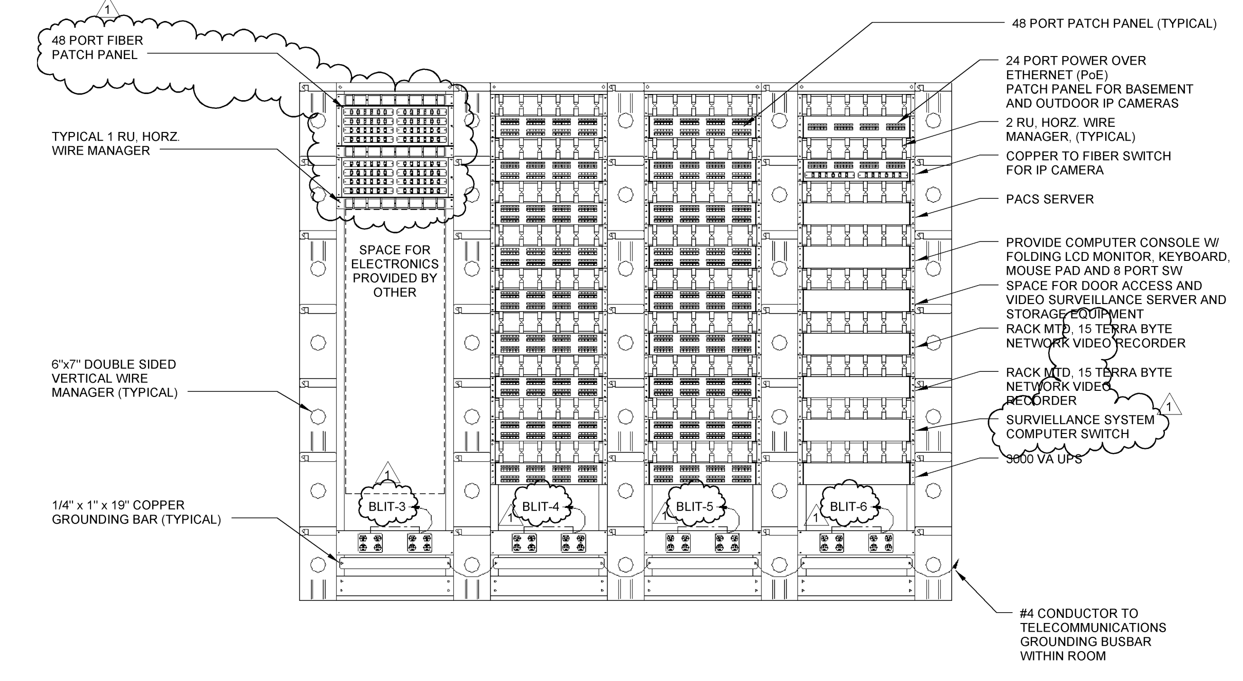
3 BASEMENT LEVEL TELECOMMUNICATION RACK ELEVATION NOT TO SCALE
