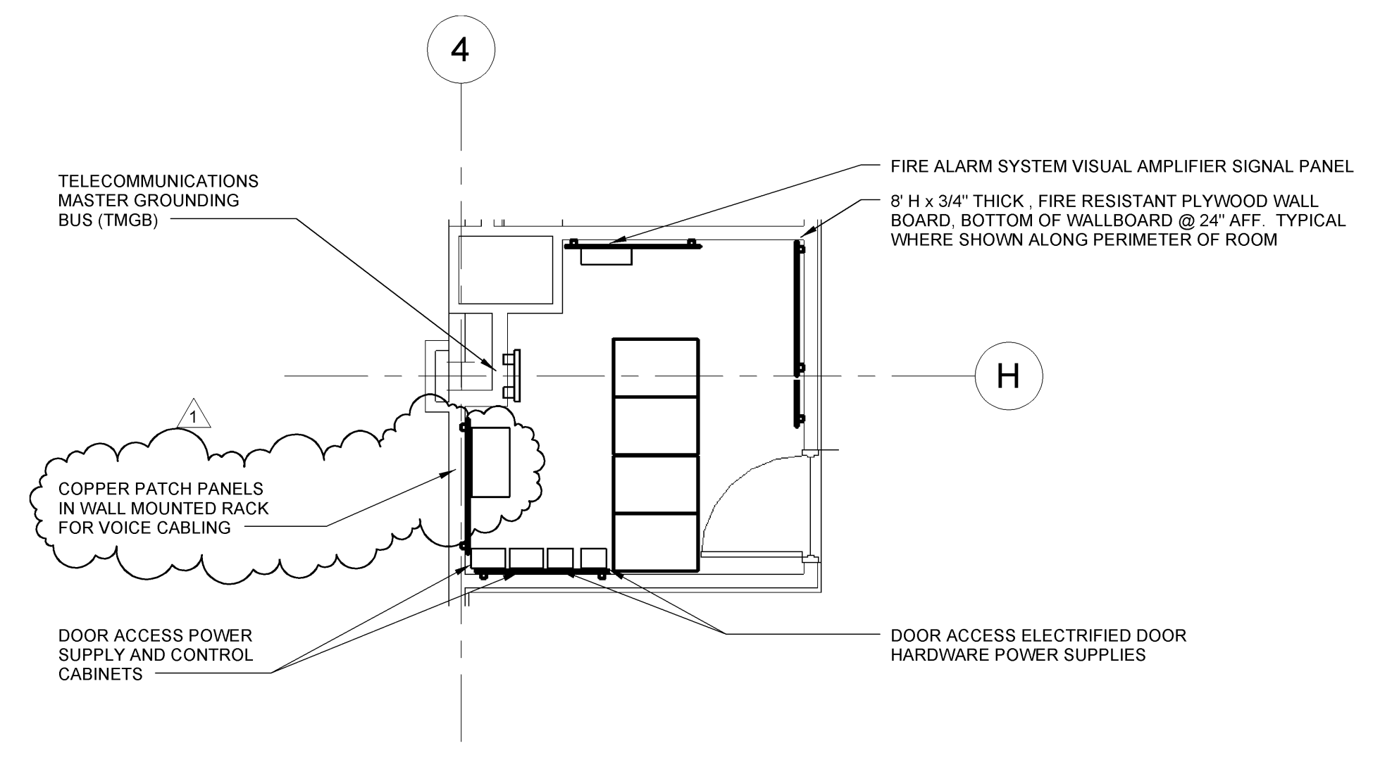
2 ENLARGED SERVICE ENTRANCE TELECOM ROOM - MDF SCALE: 1/4" = 1'-0"
