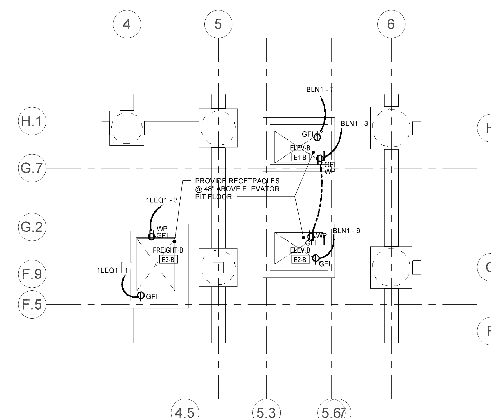
4 ELECTRICAL ELEVATOR PIT PLAN - POWER SCALE: 1/8" = 1'-0"
