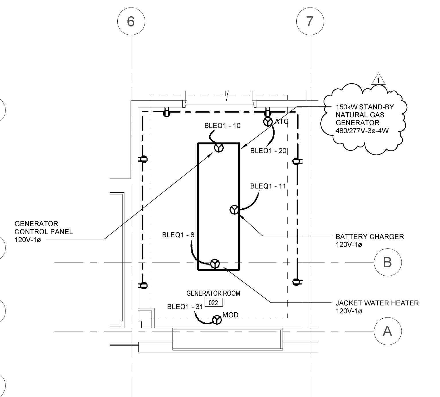
3 ENLARGED ELECTRICAL PLAN VIEW - GENERATOR ROOM SCALE: 1/4" = 1'-0"
