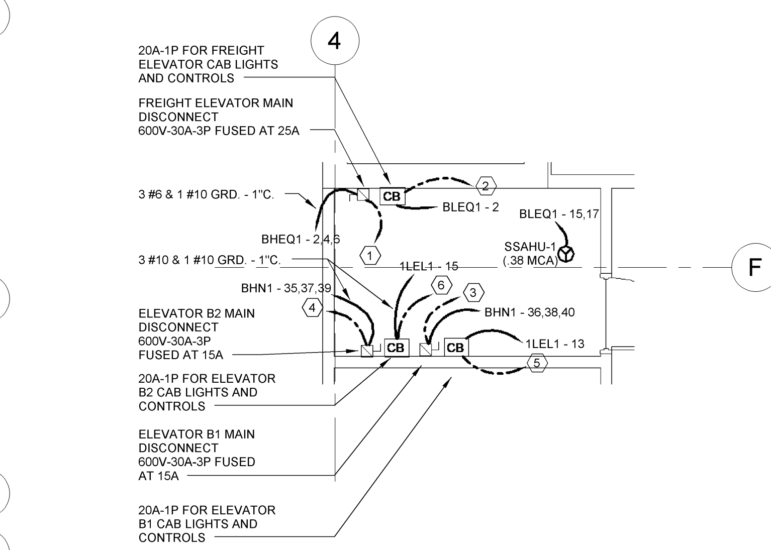
5 ENLARGED ELEVATOR MACHINE ROOM PLAN SCALE: 1/4" = 1'-0"
