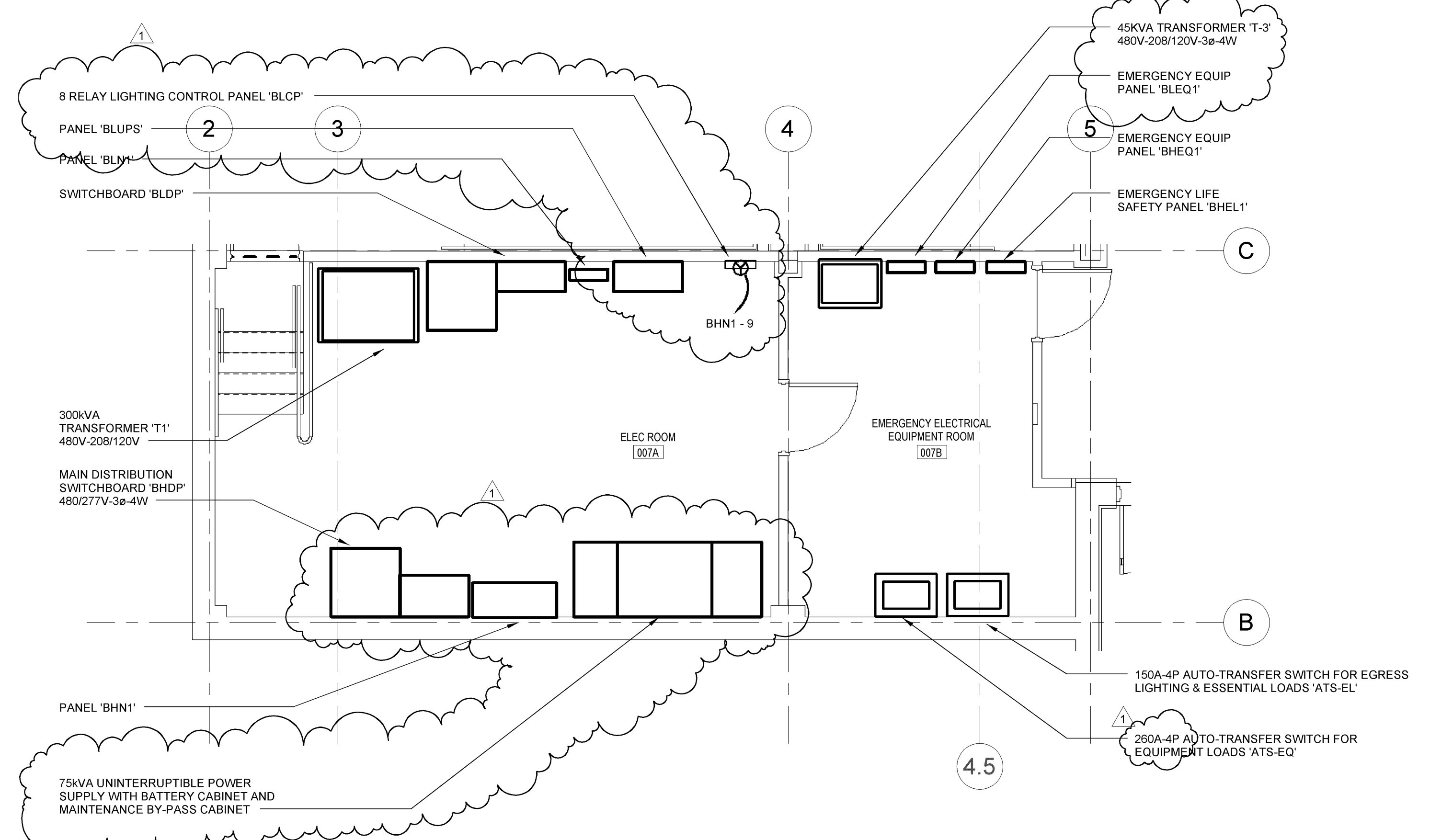
2 ENLARGED ELECTRICAL PLAN VIEW - MAIN ELECTRIC ROOM SCALE: 1/4" = 1'-0"
