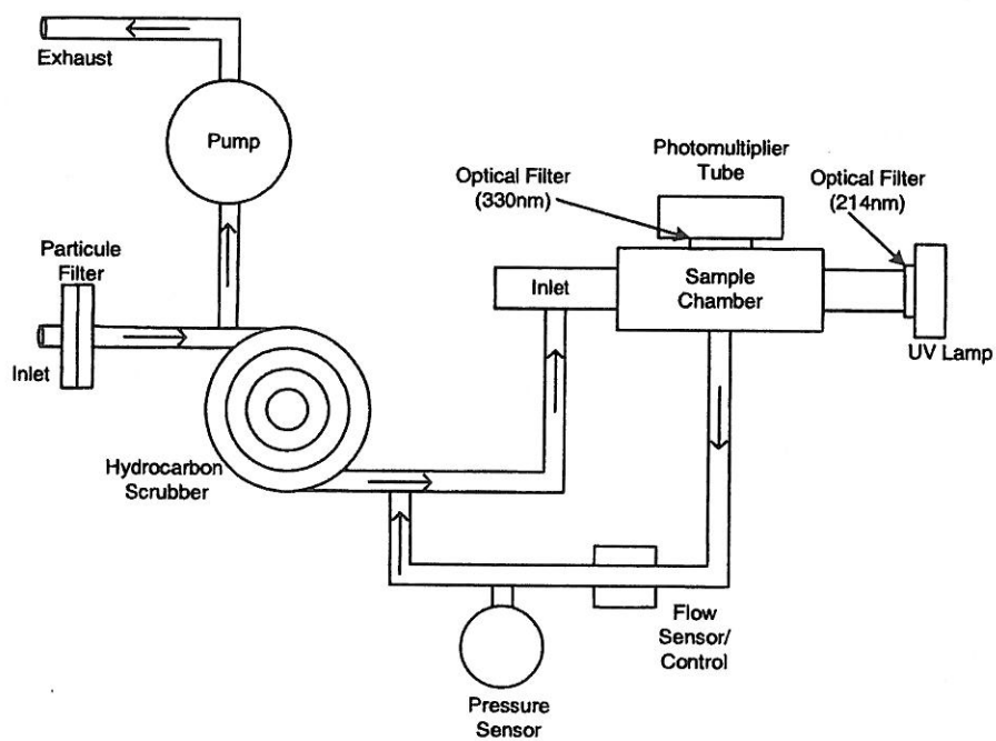
Figure 1. UVF SO 2 analyzer schematic diagram.
