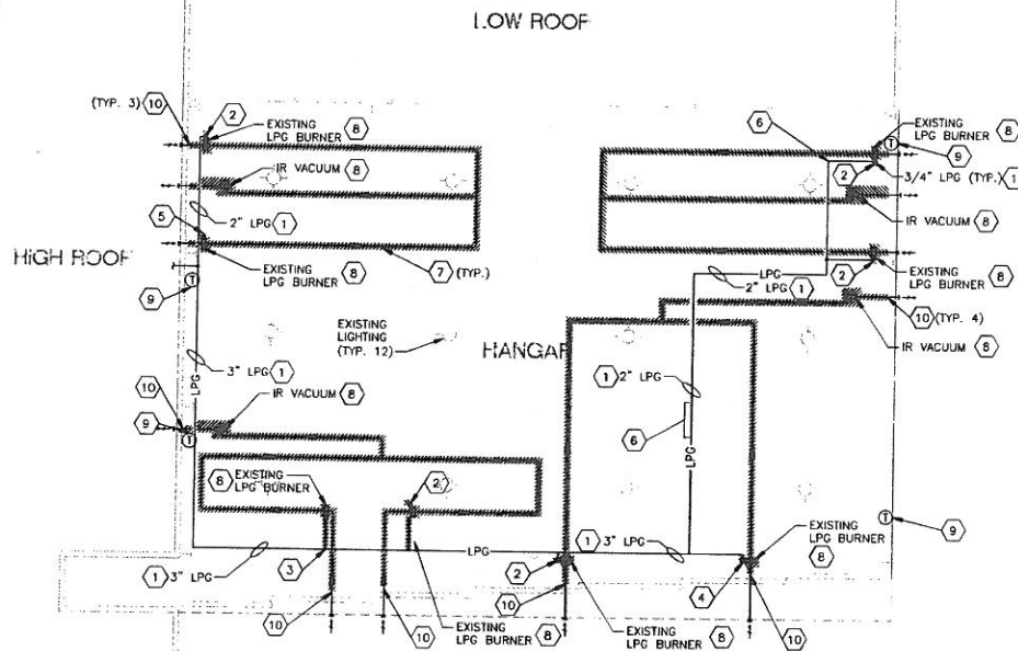
HANGAR IR-HEATER DEMOLITION PLAN DATE 10-1-10
