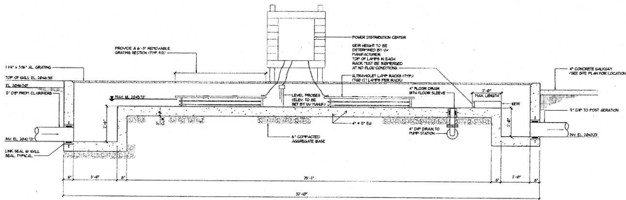
ULTRAVIOLET DISINFECTION SYSTEM SECTION SCALE: 1/4\"/>
