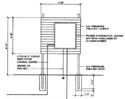
POWER DISTRIBUTION CONTROL SCHEMATIC SCALE: NONE
