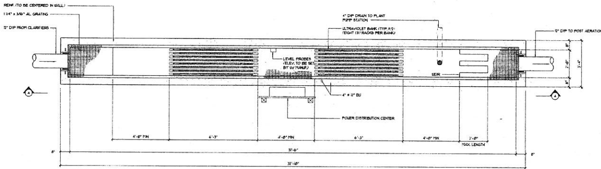
ULTRAVIOLET DISINFECTION SYSTEM PLAN SCALE: 1/4\"/>
