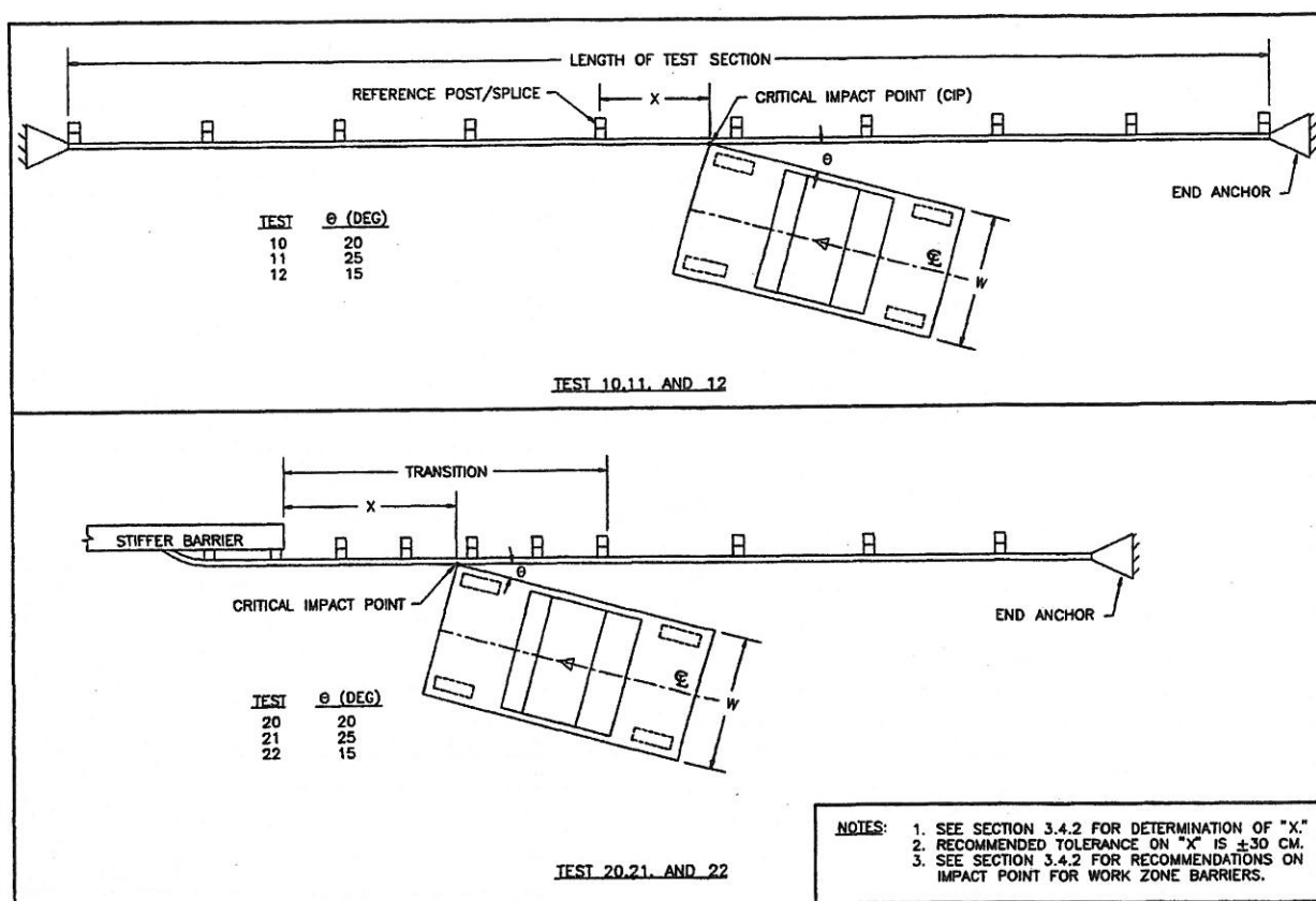
Figure 3.1. Impact conditions for longitudinal barrier tests.
