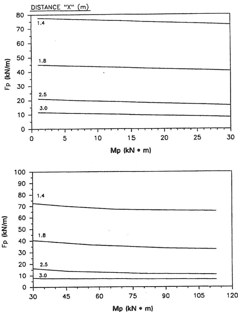
Figure 3.8. Critical impact point for Test 10, levels 3, 4, 5, and 6.
