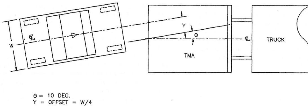
TEST NO. 53 (OPTIONAL)
