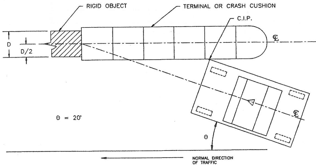
TEST 38 FOR NONGATING DEVICE WHEN D \leq 1.2 \text{ m}
