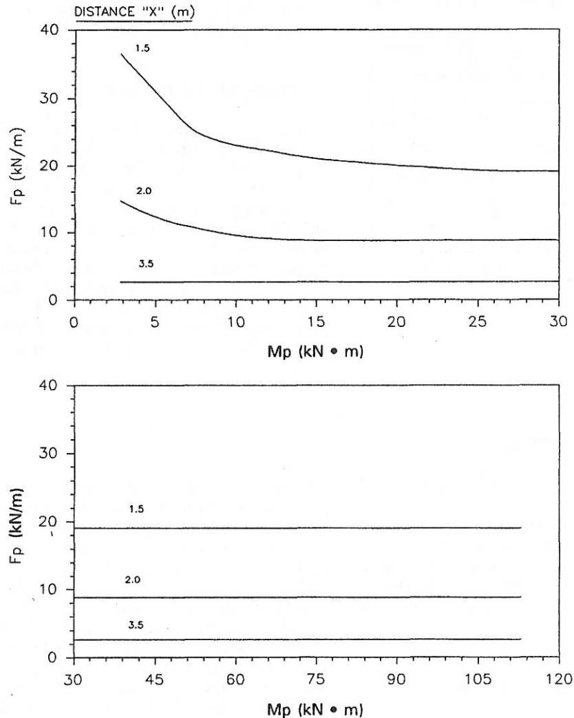
Figure 3.7. Critical impact point for Test 10, test levels 1 and 2.
