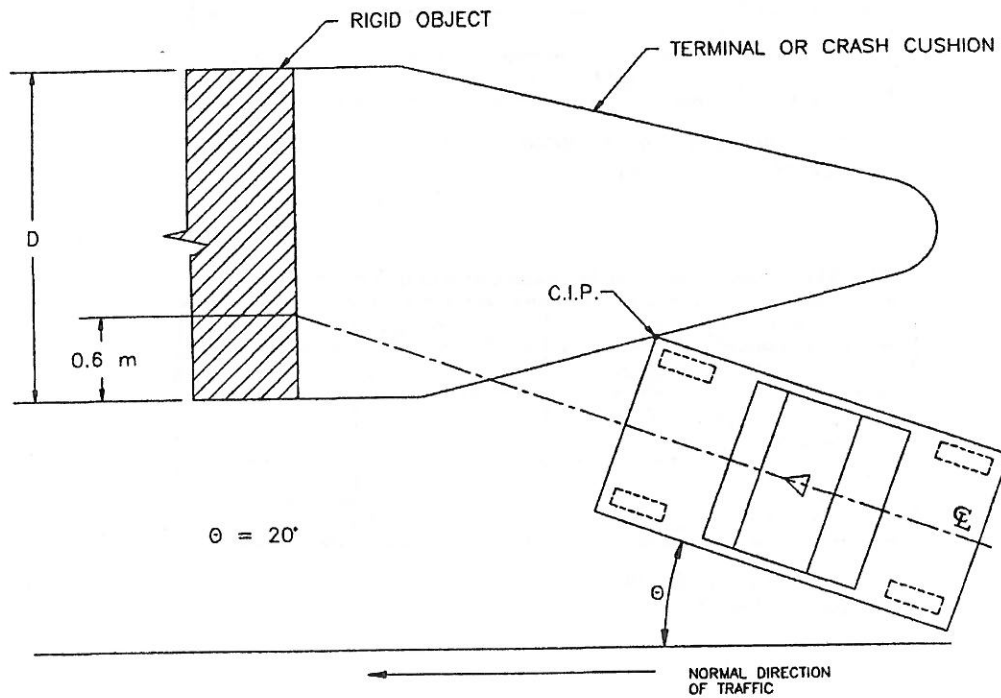
TEST 38 FOR NONGATING DEVICE WHEN D > 1.2 \text{ m}
