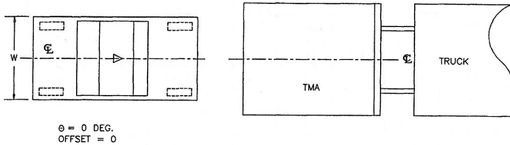
TEST NOS. 50 AND 51
