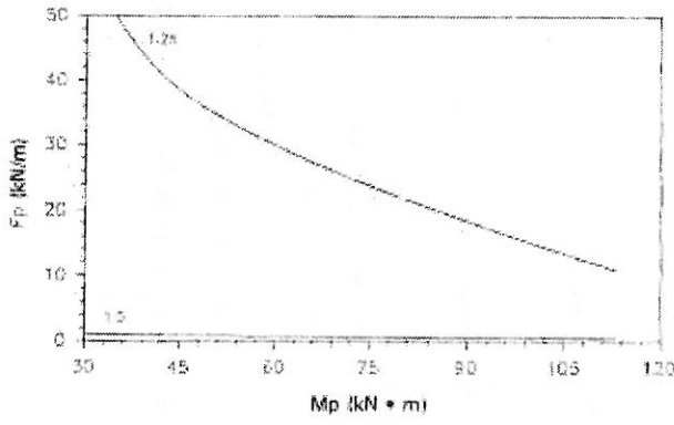
Figure 3.11. Critical impact point for Test 20, test levels 1 and 2.
