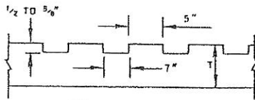
ALTERNATE SECTION B-B (SAWED RUMBLE STRIP)
