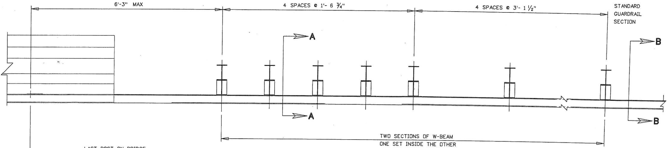
PLAN
