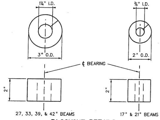
BLOCKOUT DETAILS
