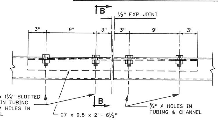
TUBING SPLICE/EXPANSION JOINT DETAIL
