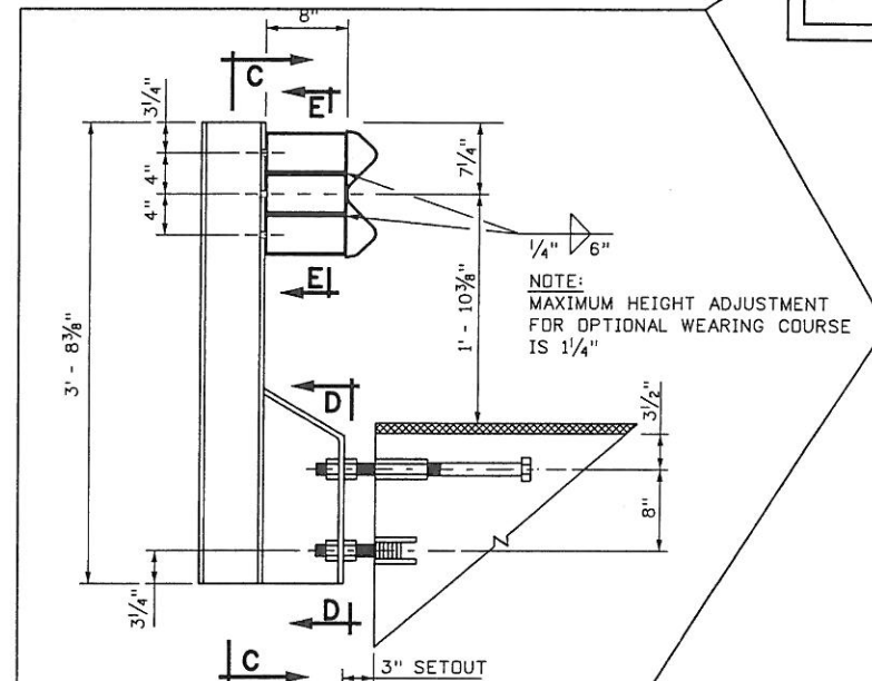
GUARDRAIL POST DETAIL "B"
