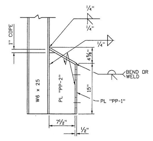
SECTION F-F
