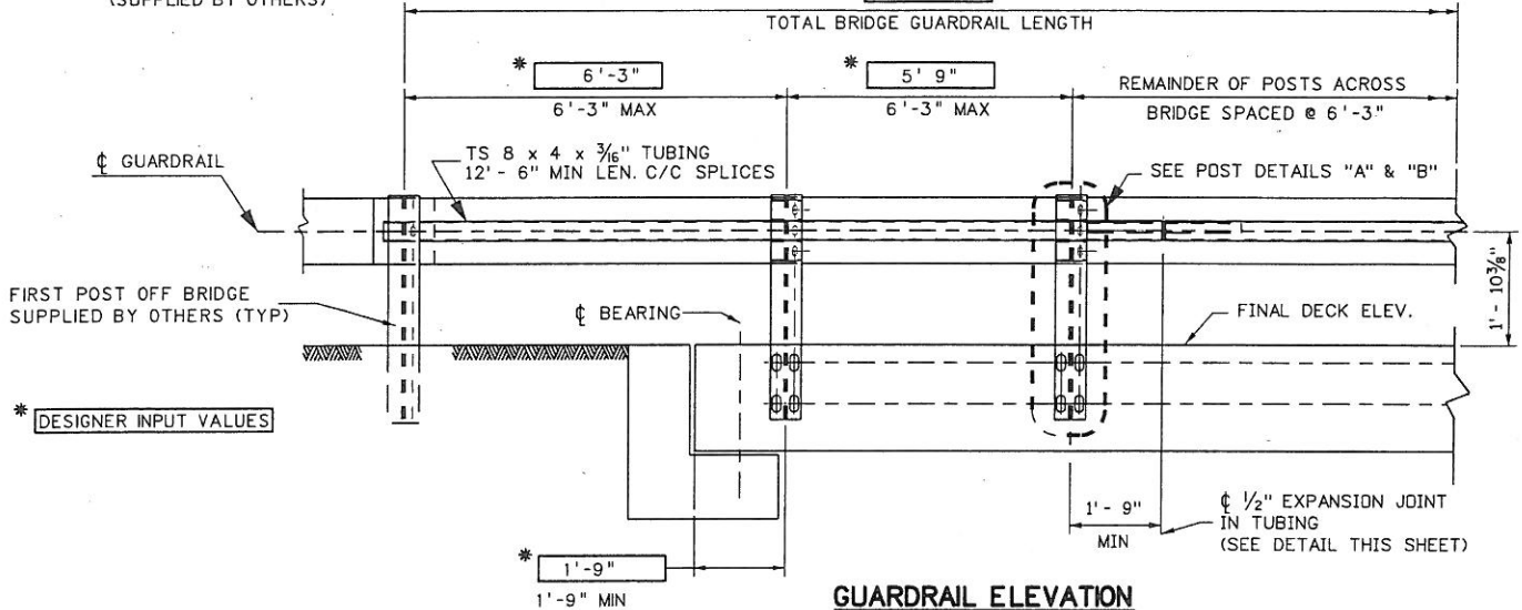
GUARDRAIL ELEVATION
