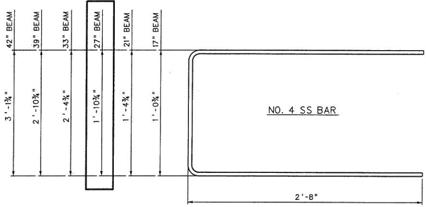
END BEARING DETAIL WITH BACKWALL
