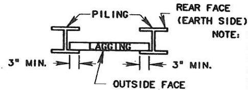
DETAIL 'A-A'
