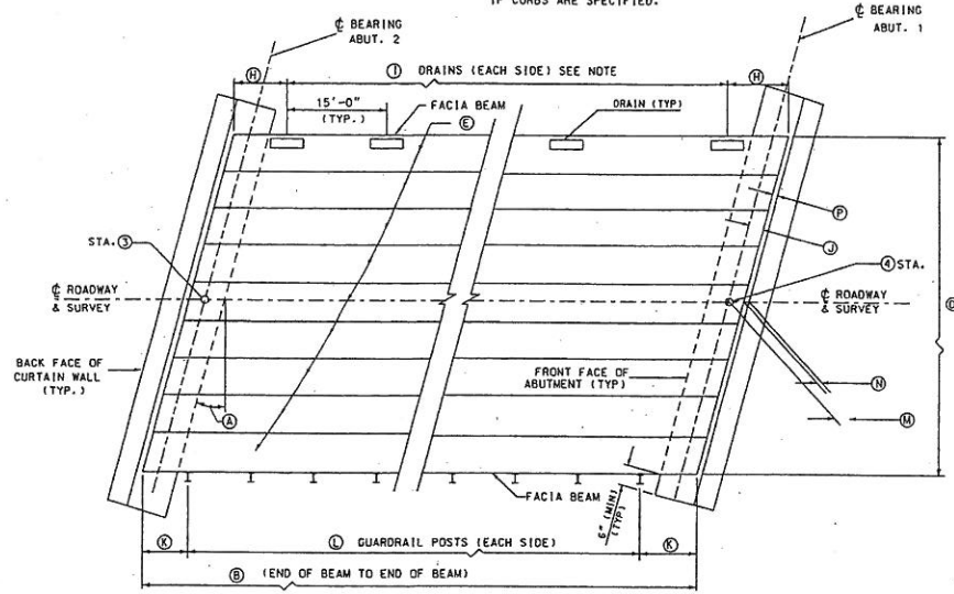
SUPERSTRUCTURE LAYOUT PLAN
