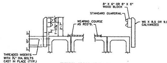
TYPICAL CROSS SECTION WITHOUT CURB
