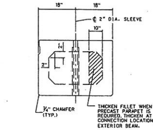
TYPICAL END BEARING DETAIL/BACKWALL (ALONG CENTER LINE ROADWAY)
