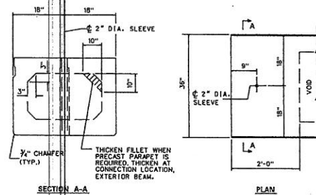
END BLOCK DETAILS
