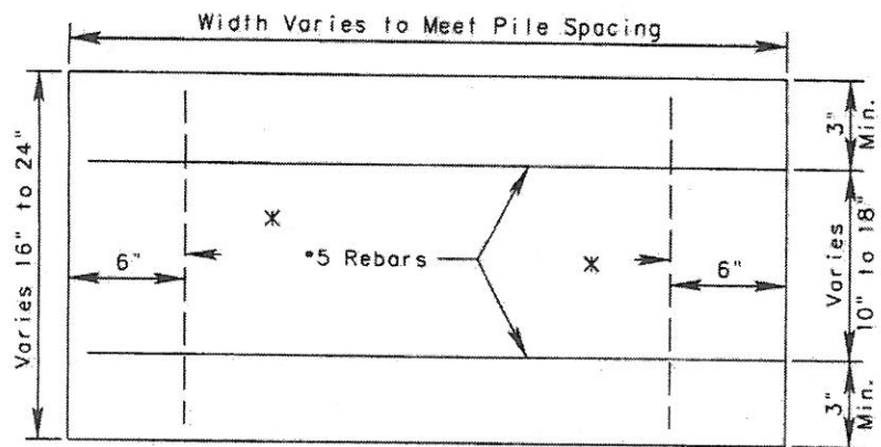
ELEVATION VIEW
