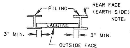
DETAIL 'A-A'
