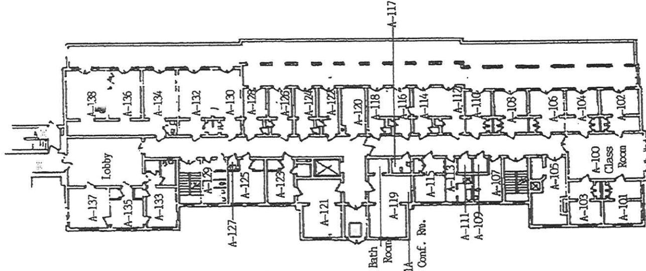
FIRST FLOOR PLAN - WING "A"
