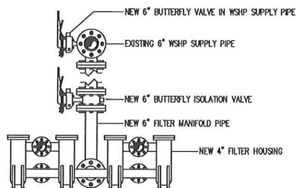
M 1b ELEVATION SECTION A-A 1"=1'-0"
