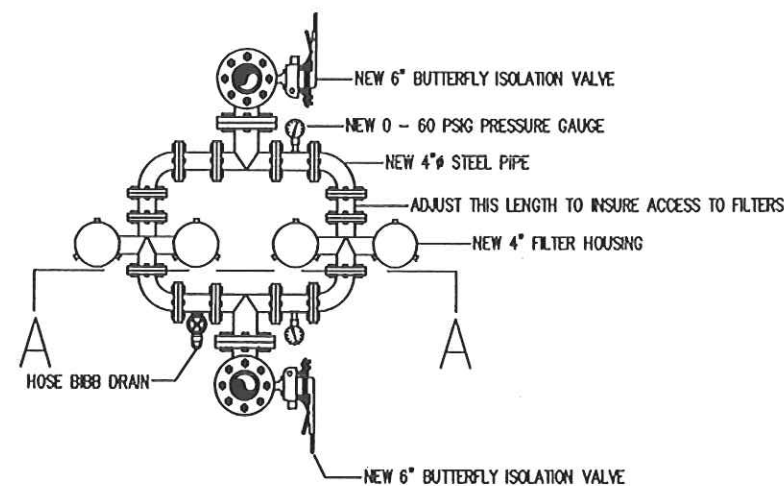
M 1a PLAN VIEW - FILTER HOUSING 1"=1'-0"
