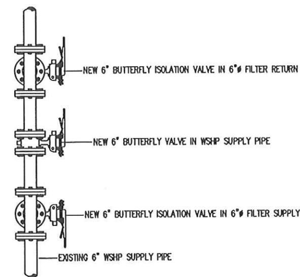
M 1c PLAN VIEW - EXISTING PIPE 1"=1'-0"
