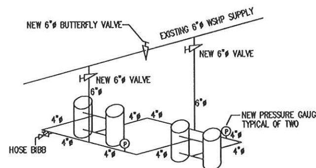
M 1d SCHEMATIC VIEW NTS
