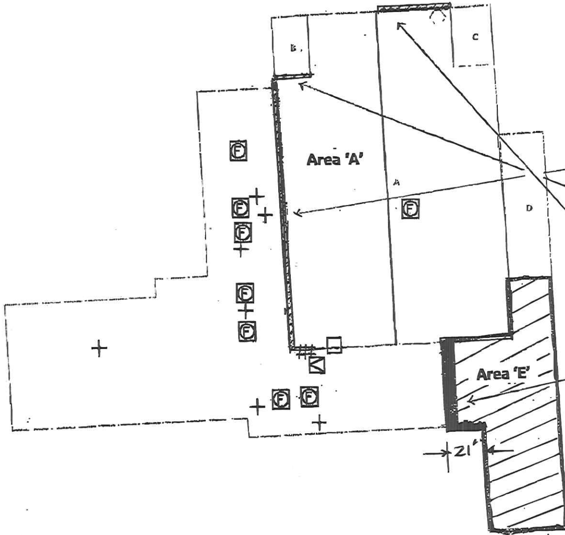
WESTON ARMORY ENTIRE ROOF SCHEMATIC Not To Scale
