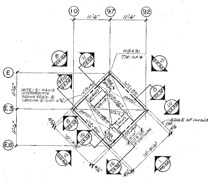
CONTROL TOWER TYP. STAIR FRAMING PLAN 1/8" = 1'-0" 1. DESIGN LIVE LOAD: 80 P.S.F. 2. TOP OF STEEL ELEVATION AS SHOWN ON ELEVATIONS 163'11.4", 163'11.4" & 163'11.4" 3. STEEL LANDING CONSTRUCTION: 2" RIGID INSULATION WITH 1/2" METAL DECK WITH 1/2" METAL DECK. 4. REFERENCED: COL. SCHEDULE - S311 COL. SCHEDULE - S312
