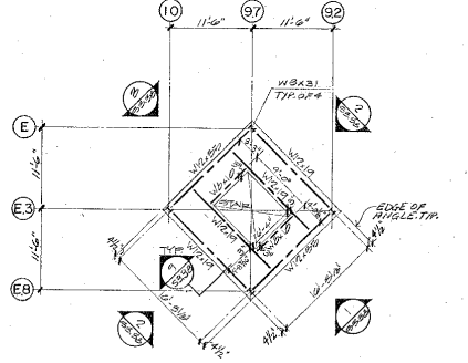
CONTROL TOWER FLOOR FRAMING PLAN 1/8" = 1'-0" 1. DESIGN LIVE LOAD: 80 P.S.F. 2. FINISHED FLOOR FINISHES: 80 P.S.F. 3. TOP OF STEEL ELEVATION 163'11.4" 4. FLOOR CONSTRUCTION: 4" CONCRETE SLAB ON 1 1/2" X 20 GAUGE WELD RIB COMPOSITE METAL DECK WITH 2 X 4 @ 12" O.C. & 2 #4 @ 12" O.C. 5. PROVIDE FINISHES FOR ALL EDGES OF CONCRETE SLAB ON STEEL DECKING. FINISHES TO BE AS SHOWN ON THE DRAWINGS. 6. PROVIDE BOND AND TIE-UP IF FLOOR IS TO BE CONCRETE OR SHALL BE EXPOSED. 7. CORRELATE THE STEEL CONSTRUCTION WITH THE ARCHITECTURAL DRAWINGS. 8. REFERENCED: COL. SCHEDULE - S311 COL. SCHEDULE - S312
