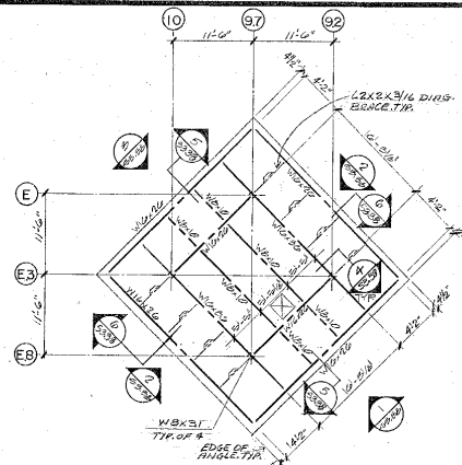
ROOF FRAMING PLAN 1/8" = 1'-0" 1. DESIGN LIVE LOAD: 800 PSF. 2. TOP OF STEEL ELEVATION 1637'-4". 3. ROOF CONSTRUCTION: 2" RIGID INSULATION WITH 1/2" METAL DECK. 4. REFERENCED: COL. SCHEDULE - S311, COL. SCHEDULE - S312.
