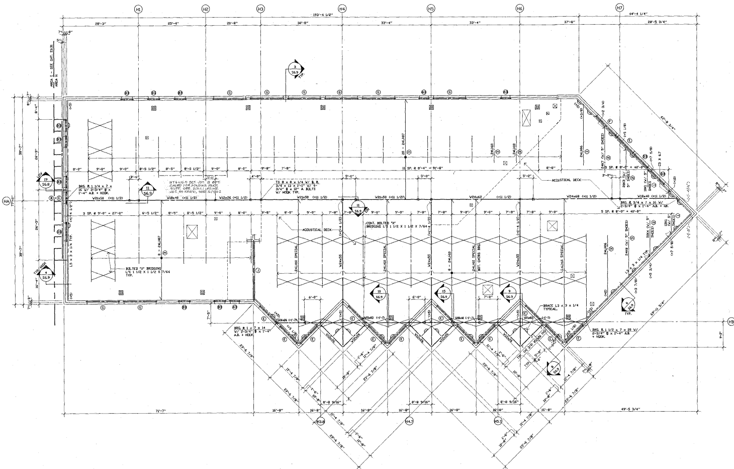
AREA H, ROOF FRAMING PLAN 1/8" = 1'-0"
