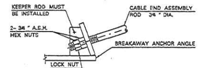
CABLE END ASSEMBLY ROD CABLE TO ANCHOR
