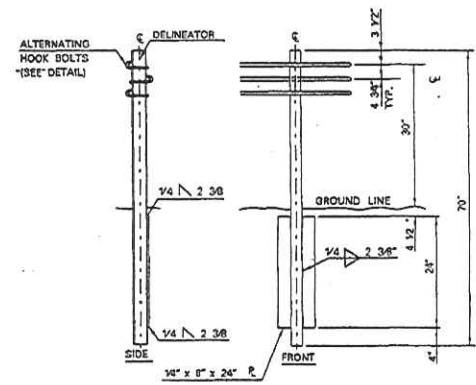
DOUBLE FACE CABLE GUARDRAIL INTERMEDIATE POST
