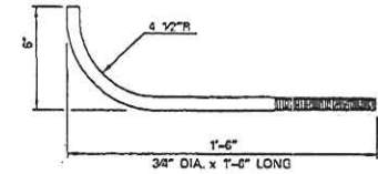
GALVANIZED ANCHOR STUD OPTION
