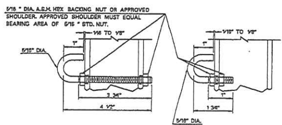
HOOK BOLT (ALTERNATES)
