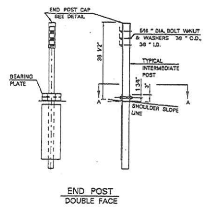
CROSSOVER END POST DOUBLE FACE
