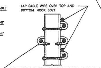
DETAIL "A" CENTER POST INTERMEDIATE ANCHORAGE SECTION
