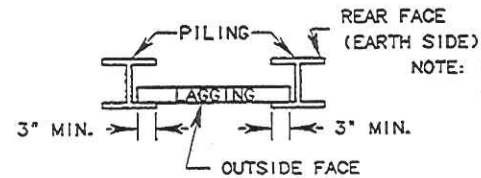
DETAIL 'A-A'
