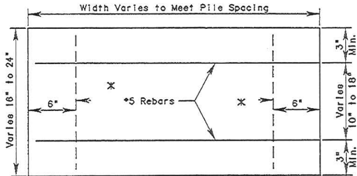
ELEVATION VIEW
