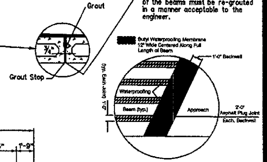
JOINT WATERPROOFING DETAIL
