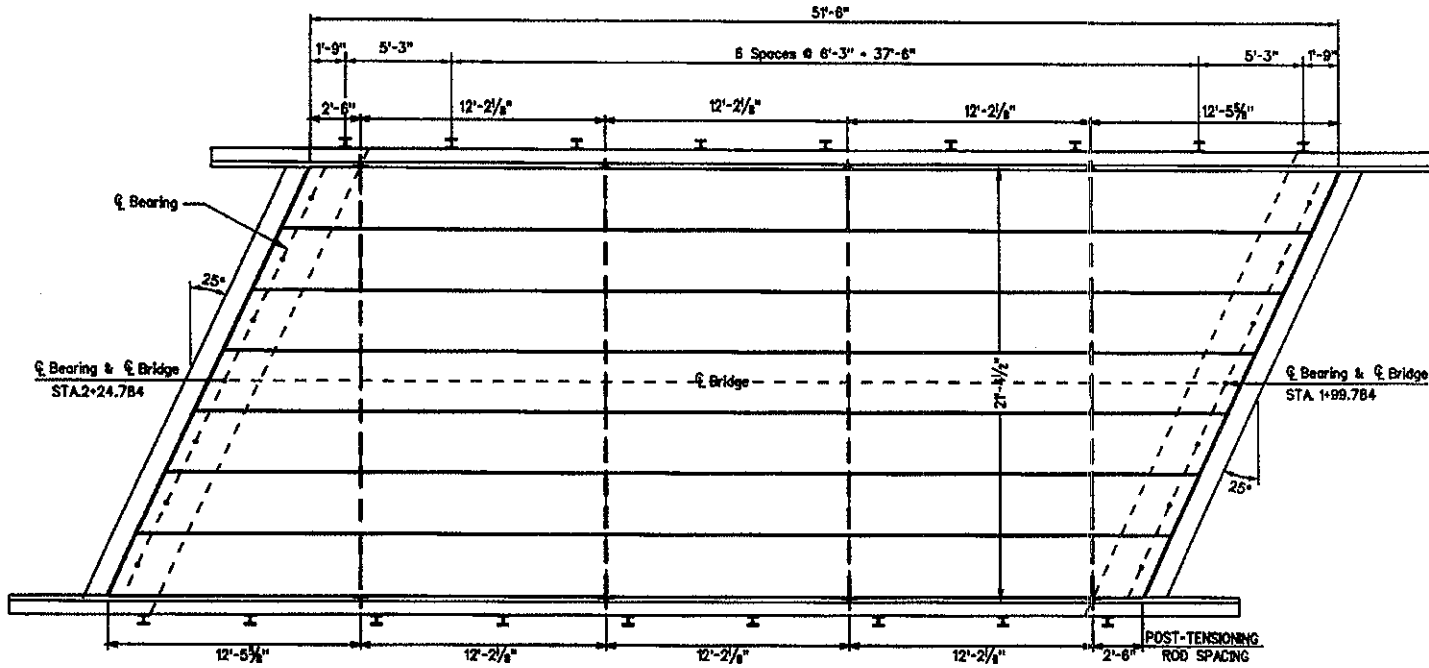
DECK PLAN
