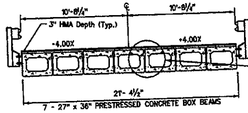
DECK SECTION
