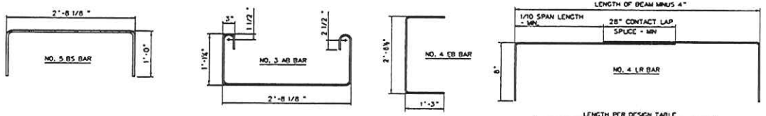
REINFORCING BAR DETAIL
