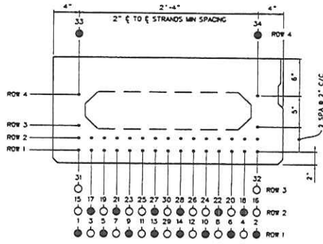
BEAM PRESTRESSING TYPICAL BEAM END & MIDSPAN
