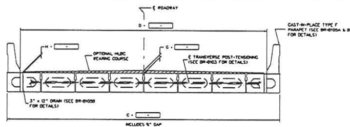
TYPICAL CROSS-SECTION WITH PARAPET OR CURB
