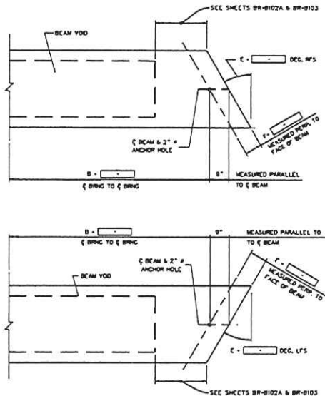
BEAM PLAN VIEW - SKEWED ENDS
