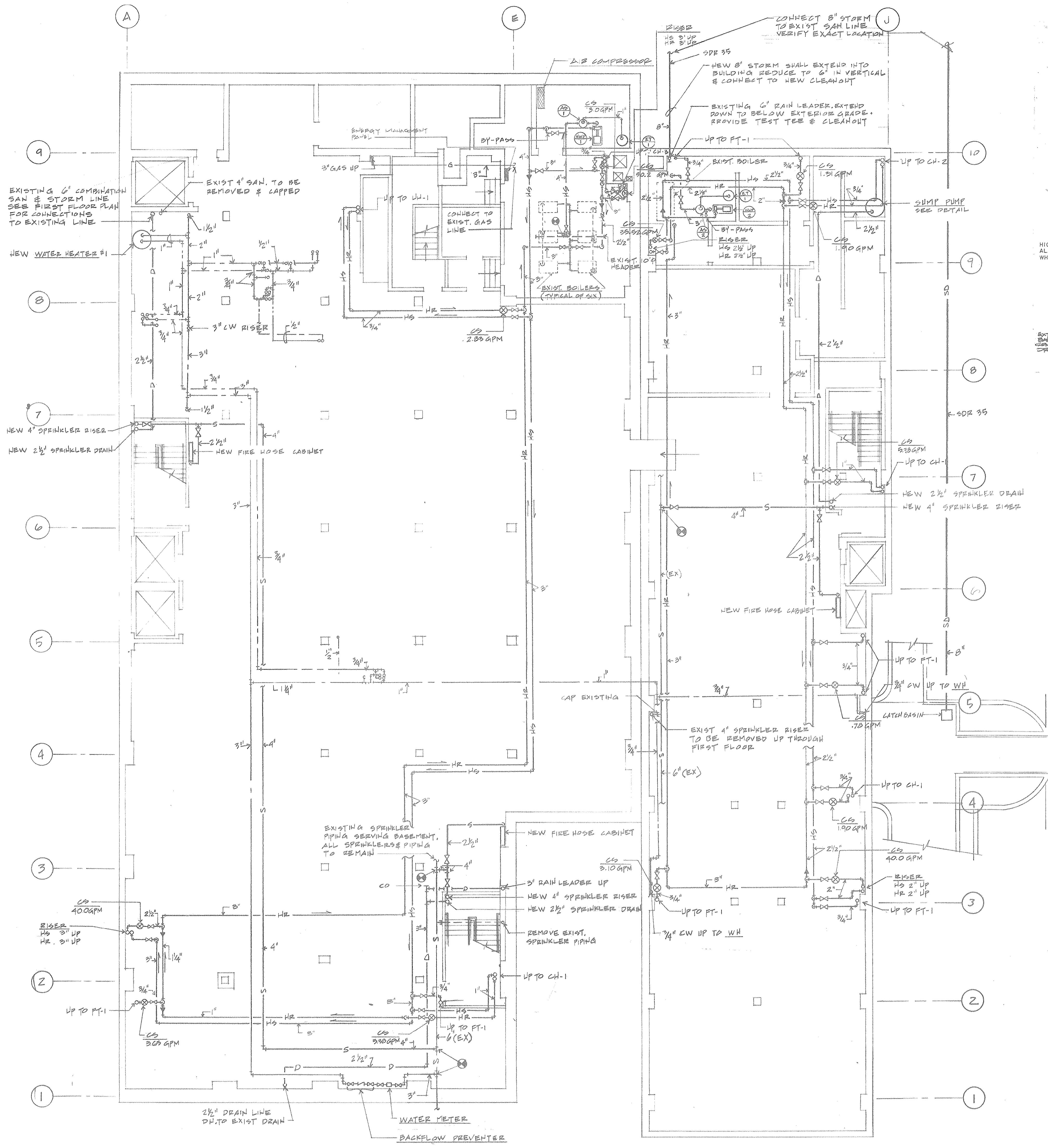
BASEMENT FLOOR PLAN - MECHANICAL SCALE 1/8" = 1'-0"
