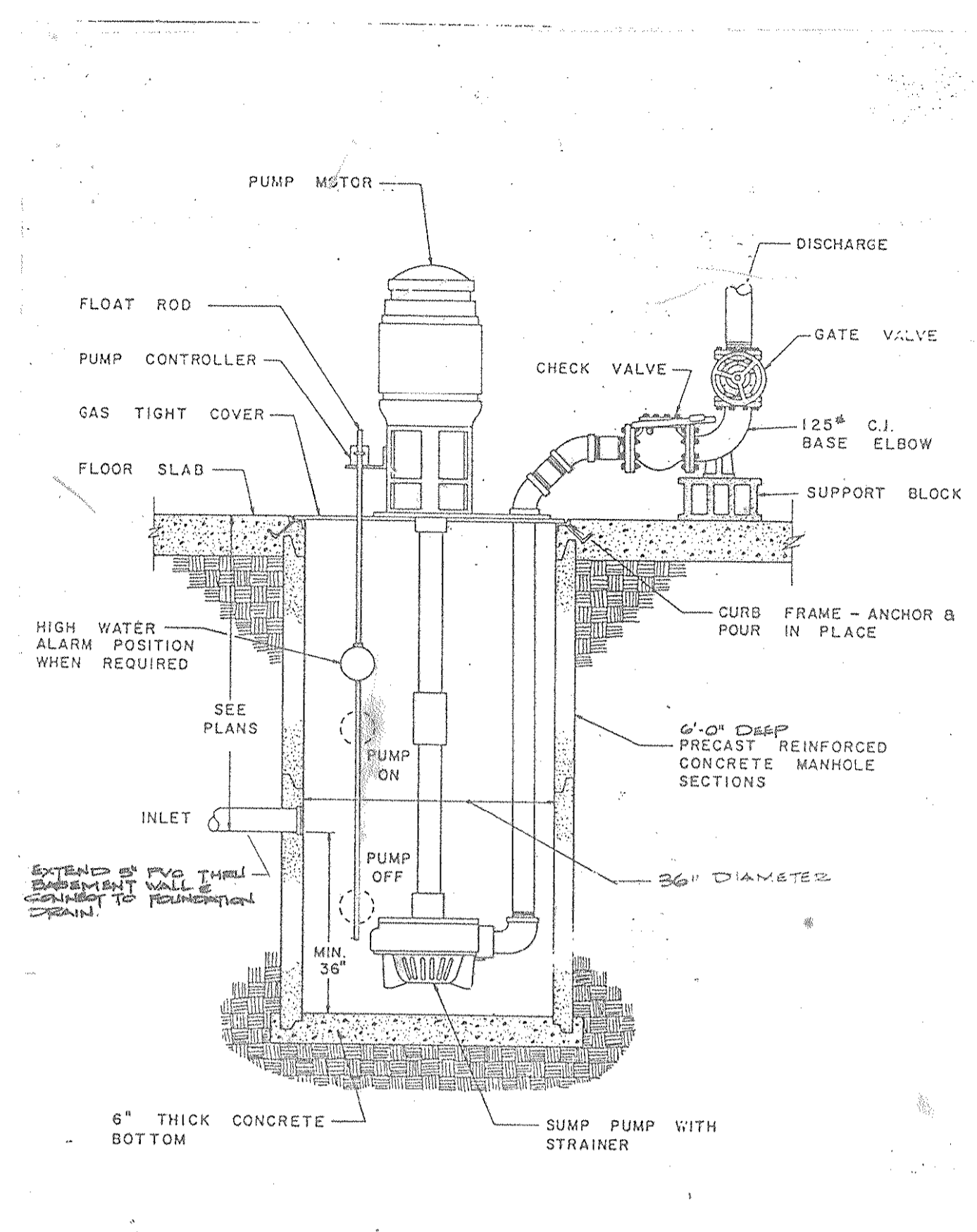
SUMP PUMP DETAIL
