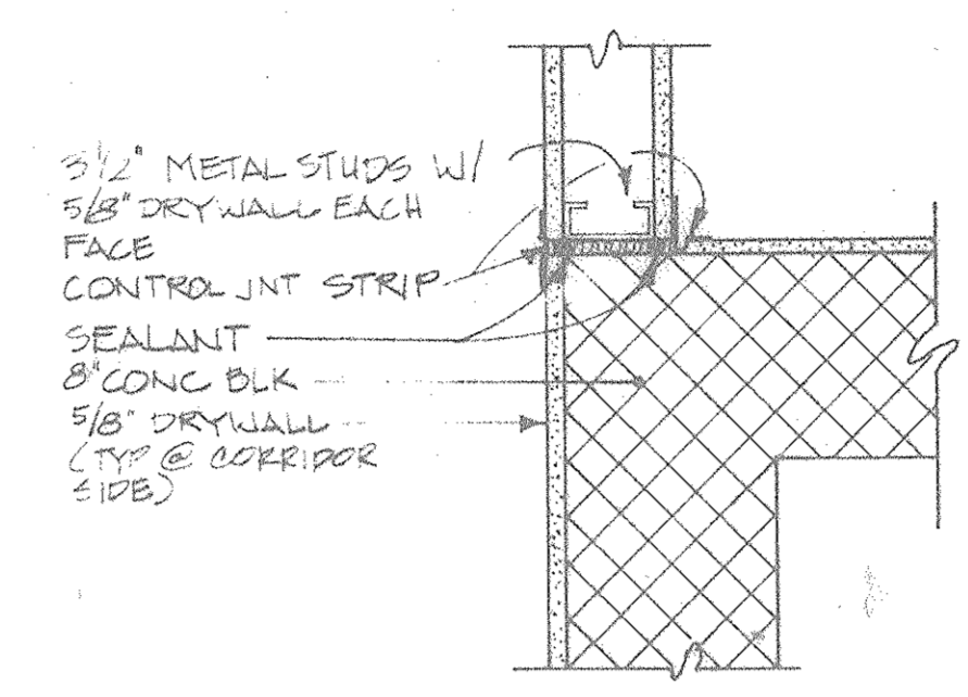
DETAIL - TYPICAL (B) SCALE 1/2" = 1'-0"
