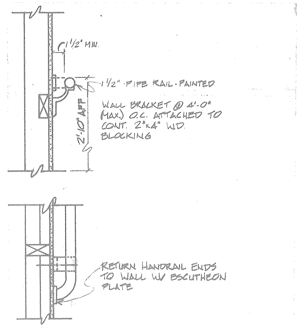
TYPICAL HANDRAIL DETAIL SCALE: 1 1/2" = 1'-0"
