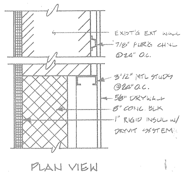
DETAIL - TYP EXT ENCLOSURE (C) SCALE 1/2" = 1'-0"
