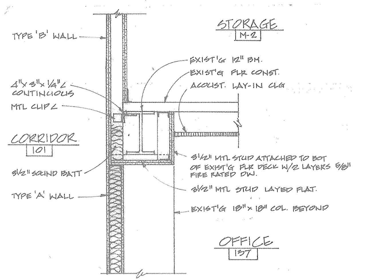
DETAIL SCALE 3/4" = 1'-0"
