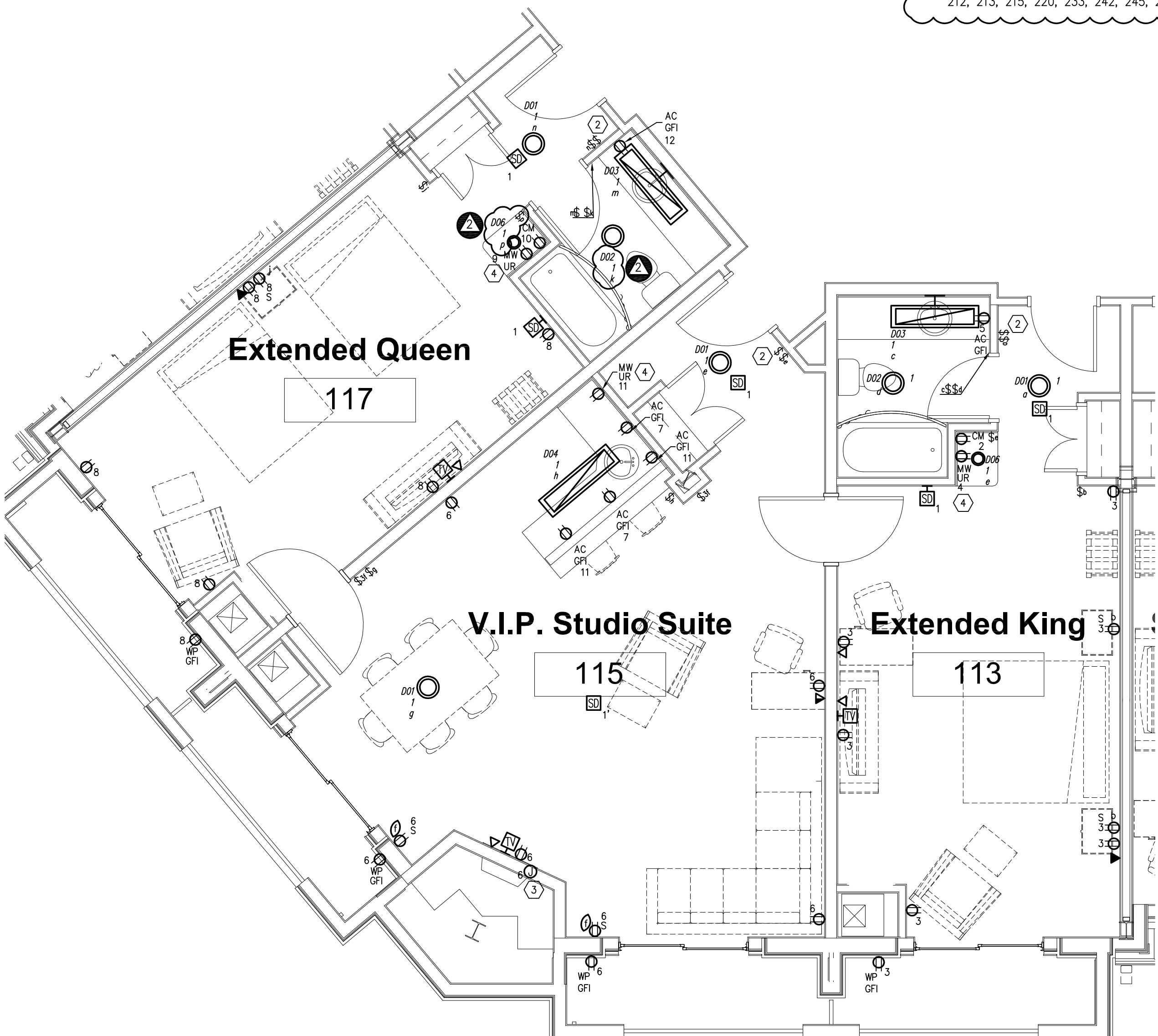
Enlarged King and Double Queen with Balcony Electrical Plan 1/4" = 1'-0"
