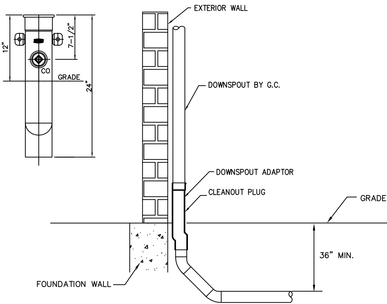
DOWNSPOUT BOOT DS-1 DETAIL NO SCALE
