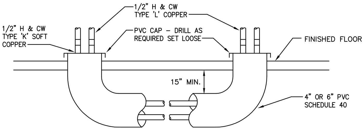
HOT & COLD WATER PIPING UNDER FLOOR SLAB DETAIL NO SCALE
