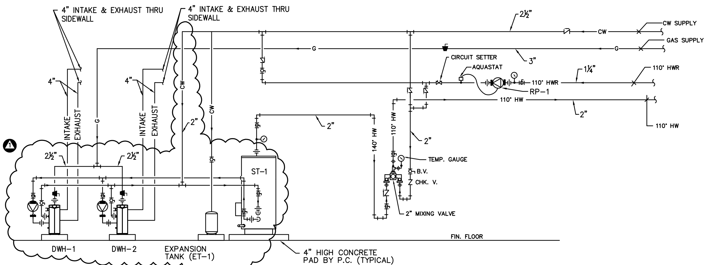
DOMESTIC WATER HEATERS (DHW-1 & DHW-2) PIPING DIAGRAM NO SCALE
