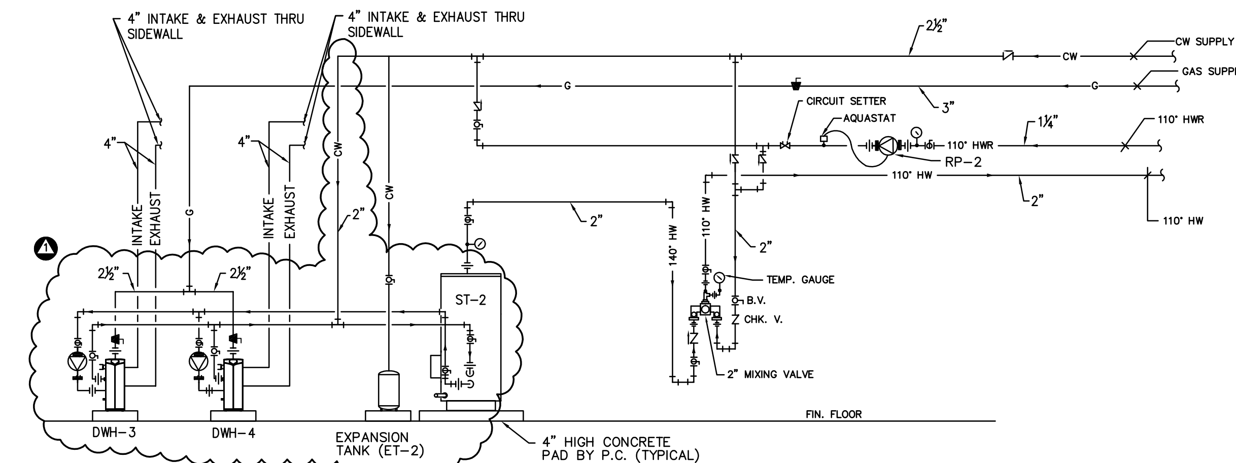
DOMESTIC WATER HEATERS (DHW-3 & DHW-4) PIPING DIAGRAM NO SCALE
