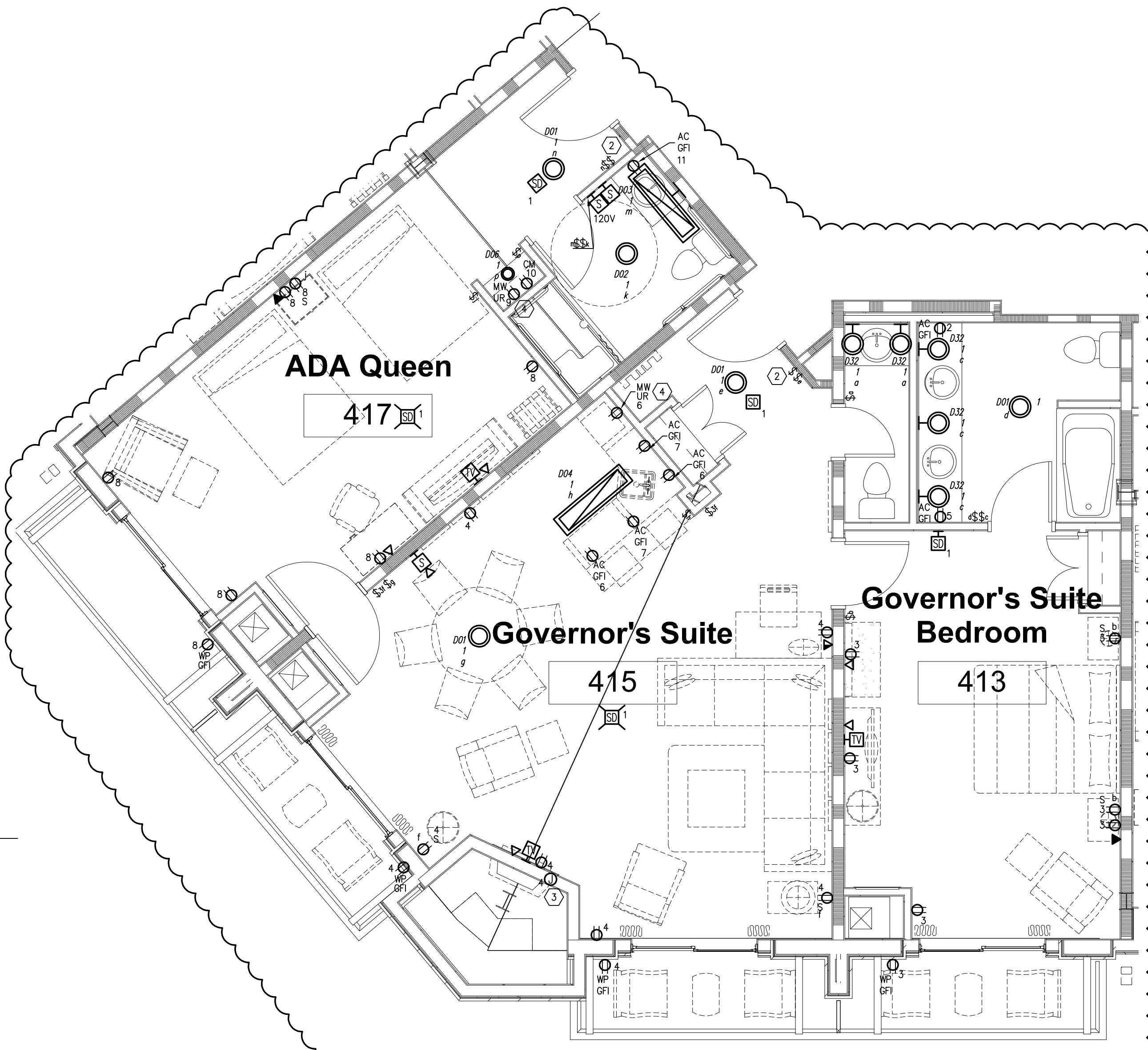
Governor's Suite Electrical Plan 1/4" = 1'-0"
