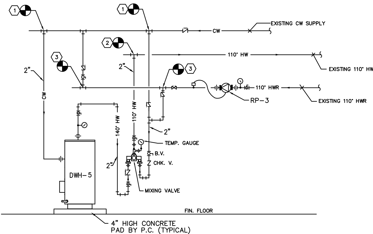
DOMESTIC WATER HEATERS (DHW-5) PIPING DIAGRAM NO SCALE
