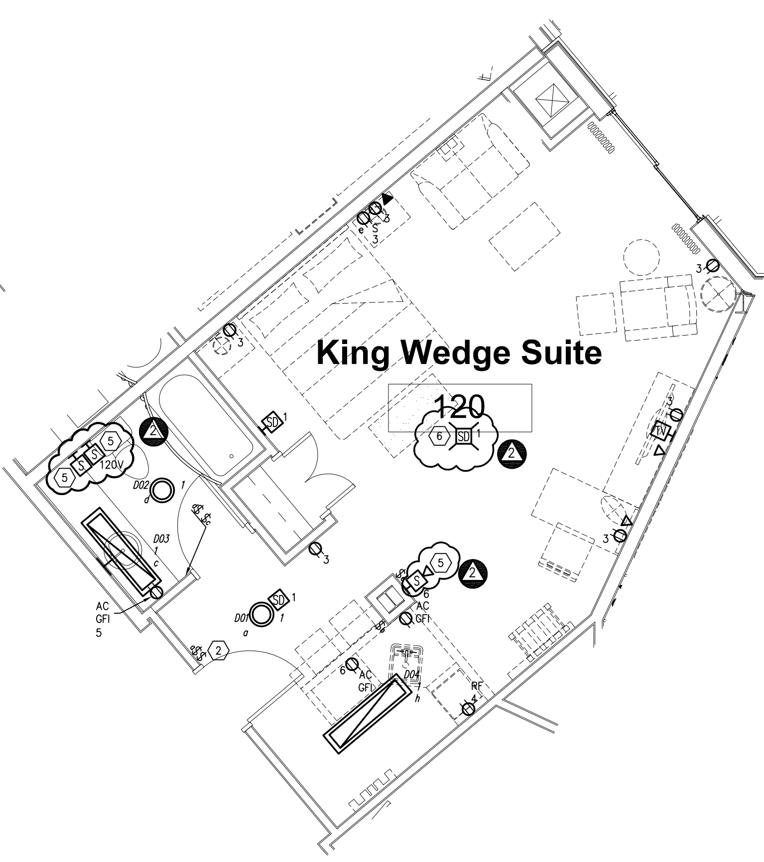
Enlarged King VIP Wedge Suite Electrical Plan 1/4" = 1'-0"
