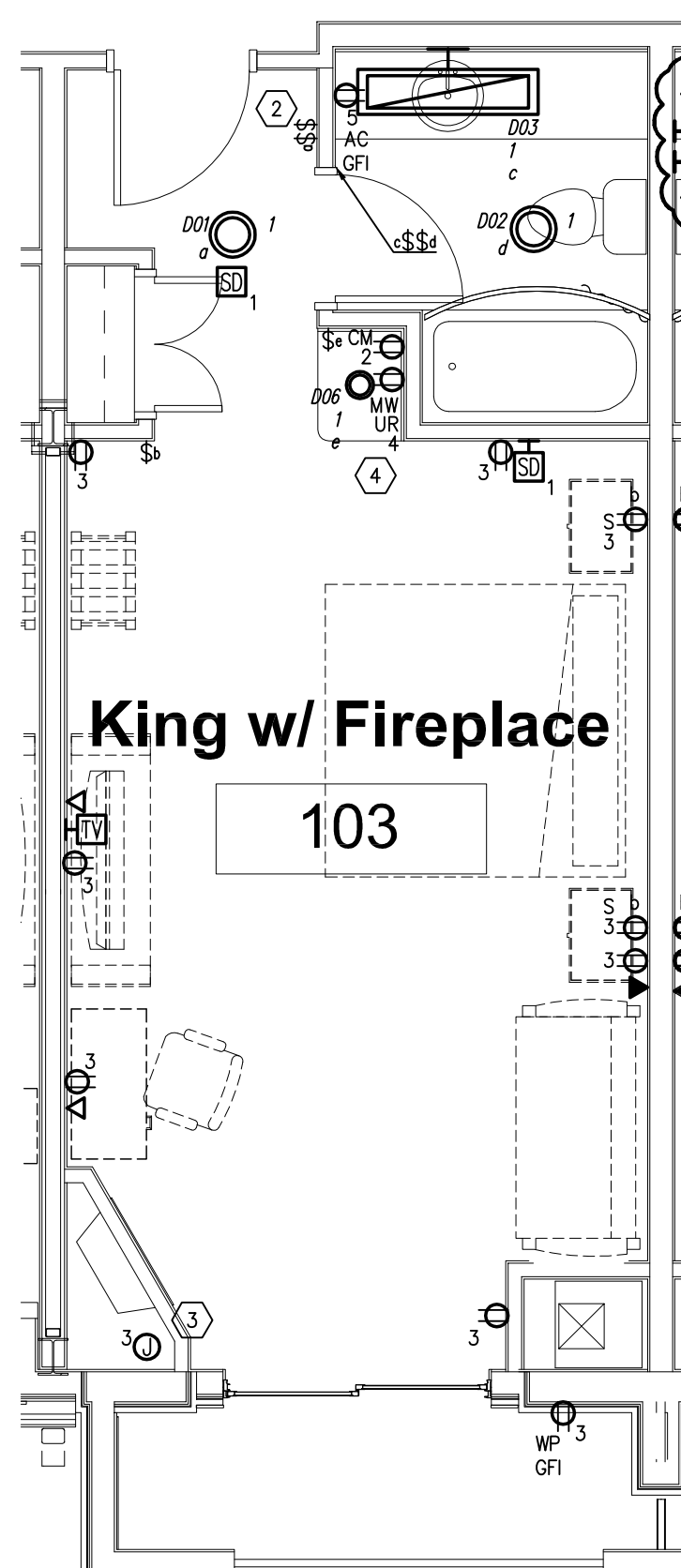
Enlarged Standard King Suite with Fireplace Electrical Plan 1/4" = 1'-0"
