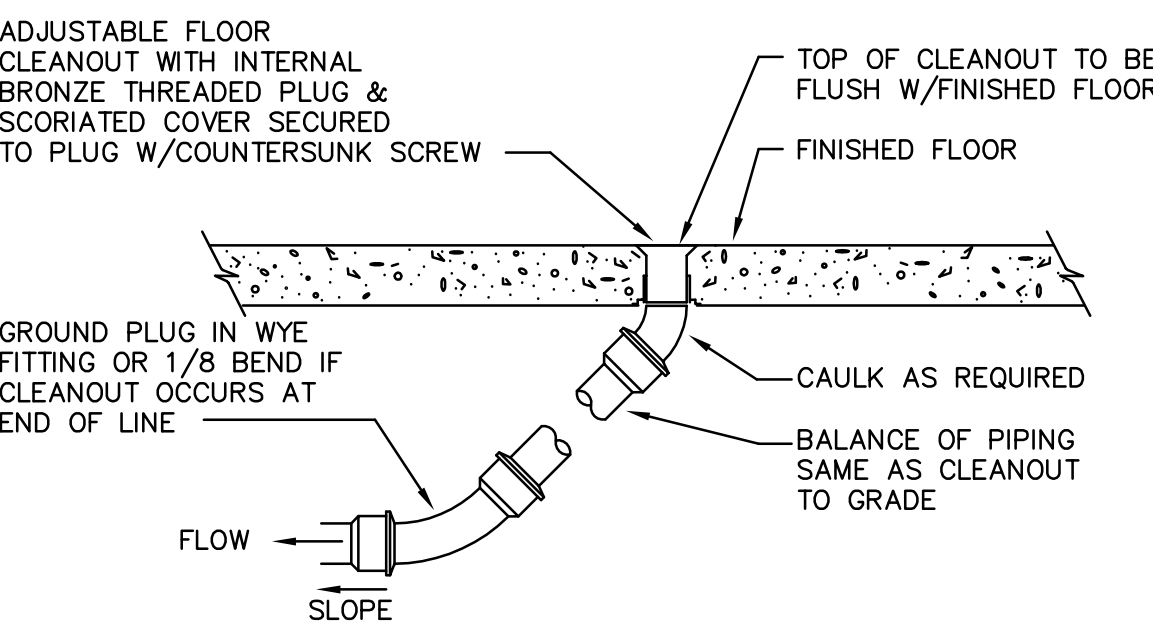
FLOOR CLEANOUT DETAIL NO SCALE
