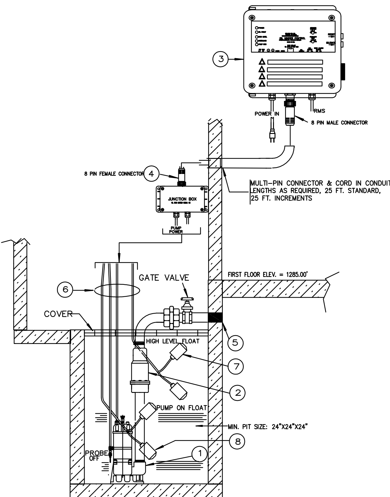
SUMP PUMP DETAIL (SP-1) NO SCALE
