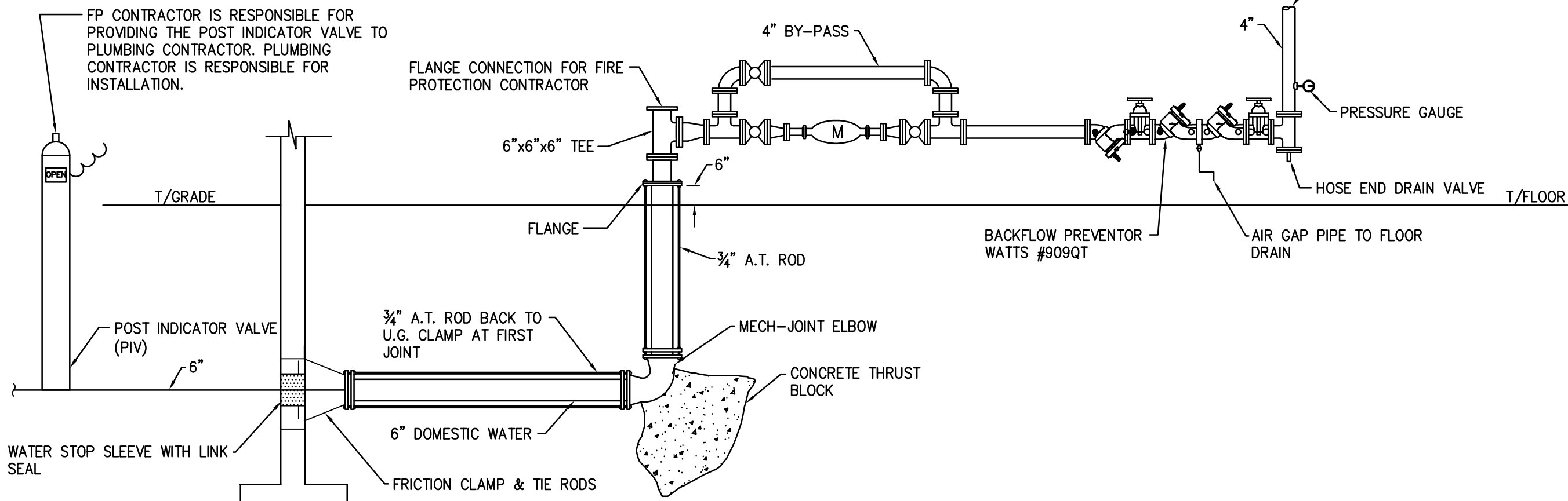
POTABLE WATER SERVICE ENTRANCE DETAIL NO SCALE
