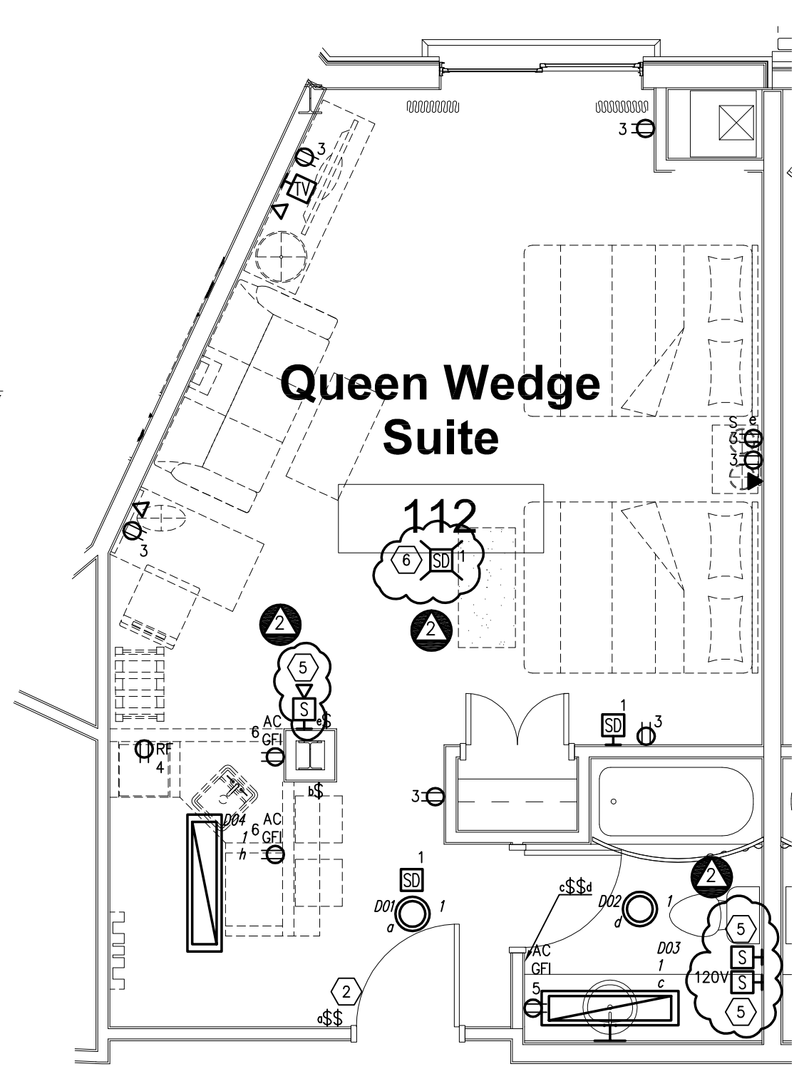
Enlarged Double Queen VIP Studio Suite Electrical Plan 1/4" = 1'-0"
