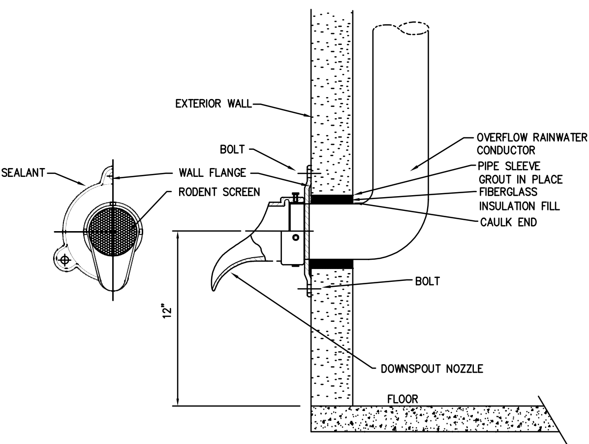
DOWNSPOUT NOZZLE (DSN-1) DETAIL N.T.S.
