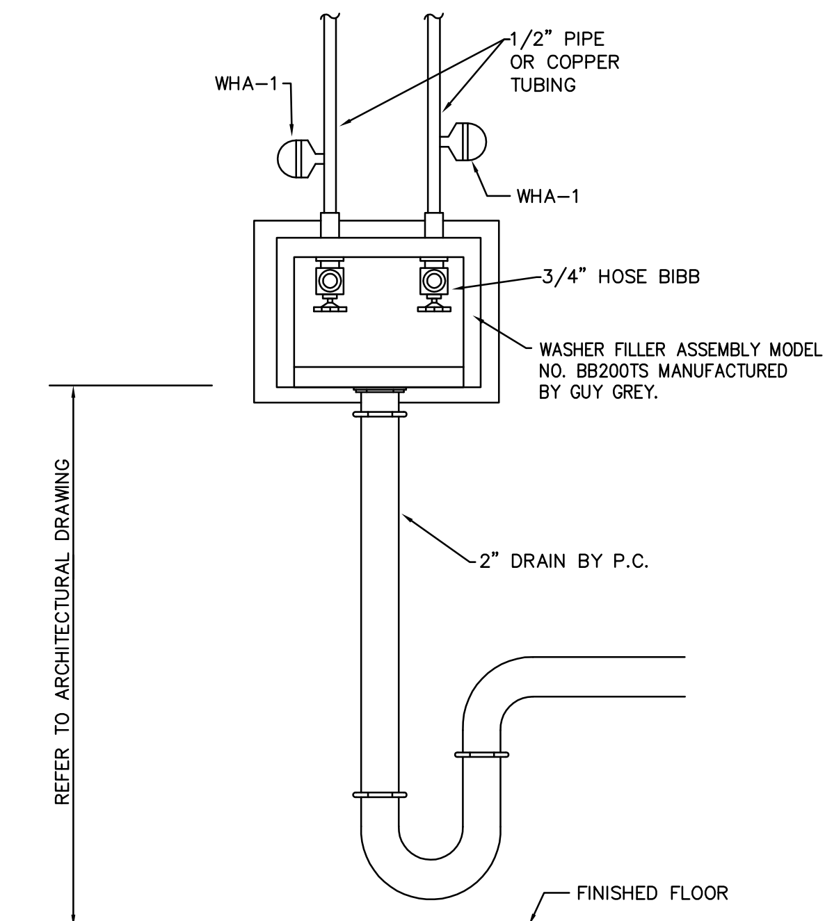
WASHER FILLER ASSEMBLY DETAIL (WFA-1) NOT TO SCALE
