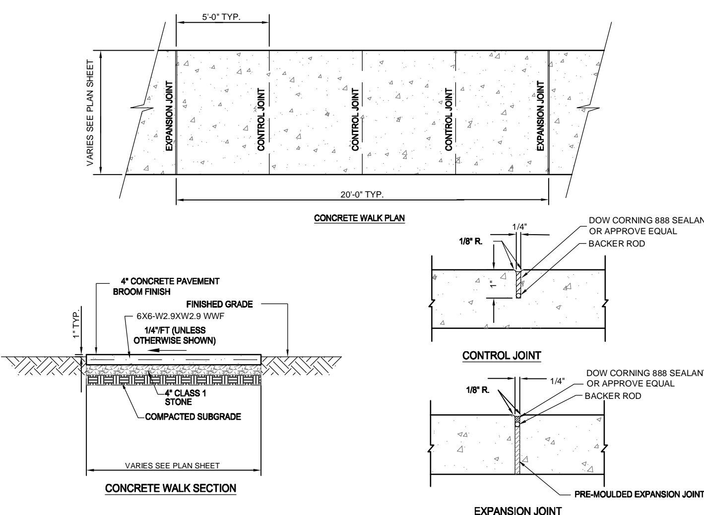
9 TYPICAL CONCRETE WALK DETAILS C801 N.T.S.
