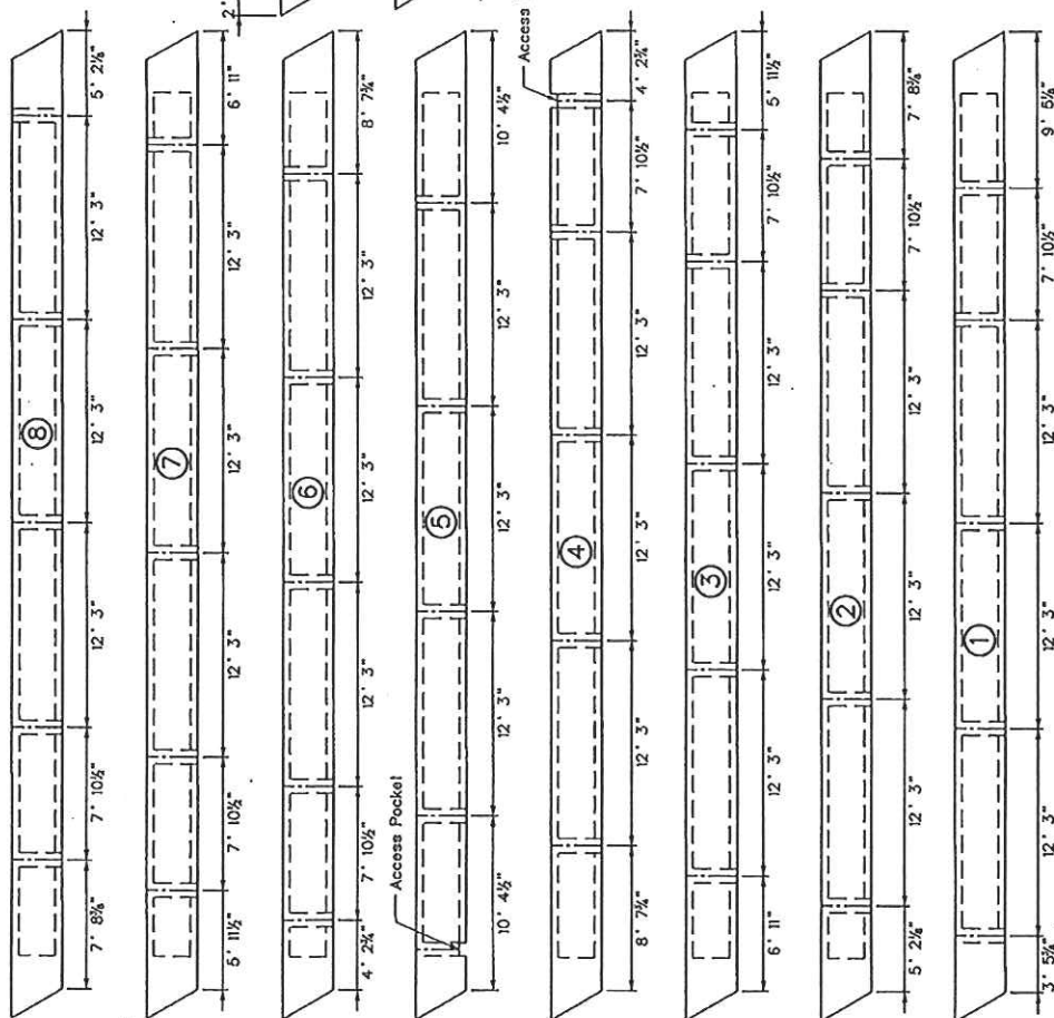
Locations of Post Tensioning Sleeves
