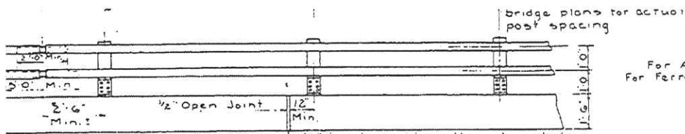
um Posts Shown ALUMINUM & FERROUS METAL BRIDGE RAILING Scale: 3/8" = 1'-0"
