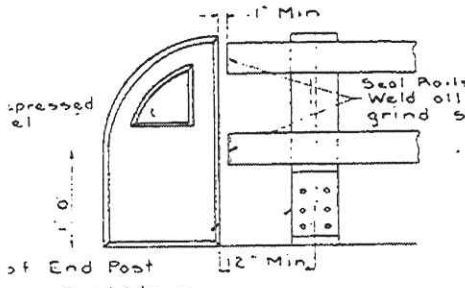
um Post Shown TERMINATION OF RAILING DETAILS Scale: 1" = 1'-0"
