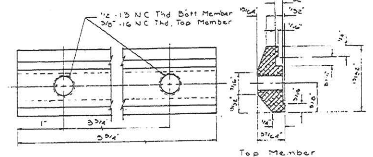
CLAMP BAR DETAILS
