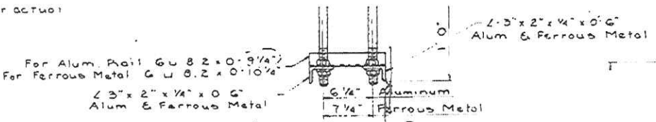
TYPICAL ANCHOR BOLT ASSEMBLY DETAIL Scale: 1/2" = 1'-0"
