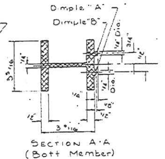
SECTION A-A (Bottom Member)
