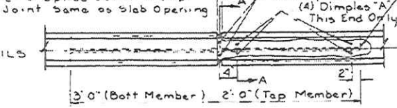
SPLICE DETAIL Scale: 1/2" = 1'-0"
