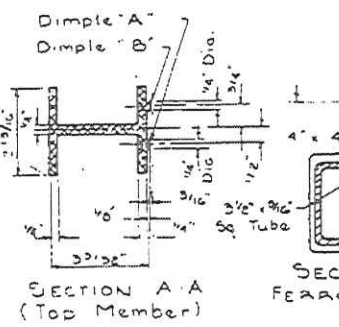
SECTION A-A (Top Member)
