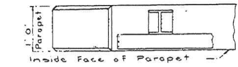
um Posts Shown ALUMINUM & FERROUS METAL BRIDGE RAILING Scale: 3/8" = 1'-0"
