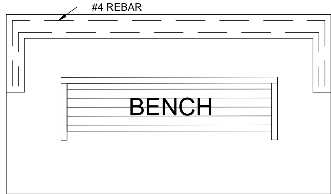
BENCH REBAR PLAN VIEW
