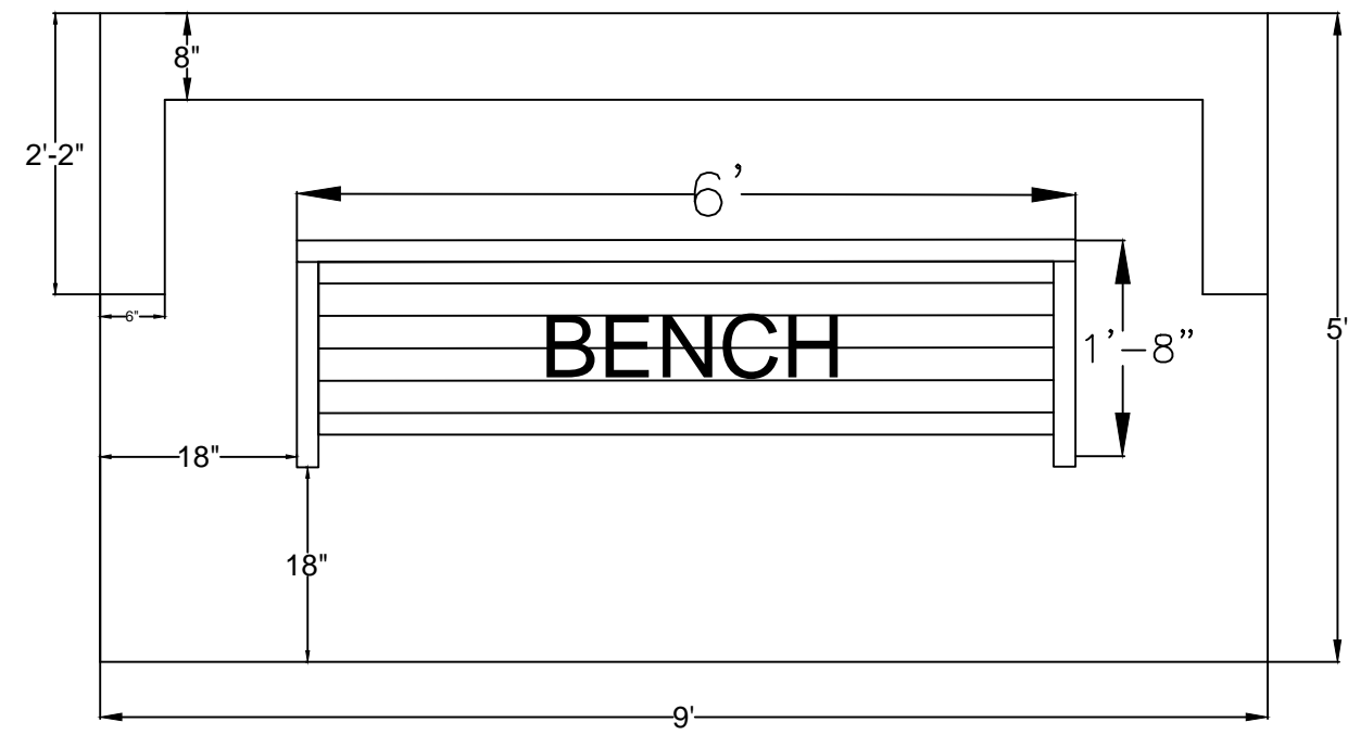
BENCH DIMENSIONS PLAN VIEW
