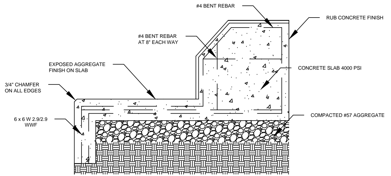
BENCH STANDARDS SECTION VIEW
