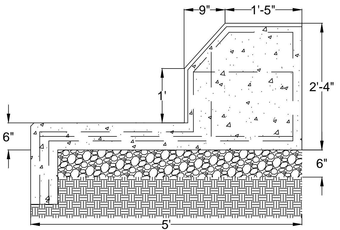
BENCH DIMENSIONS SECTION VIEW
