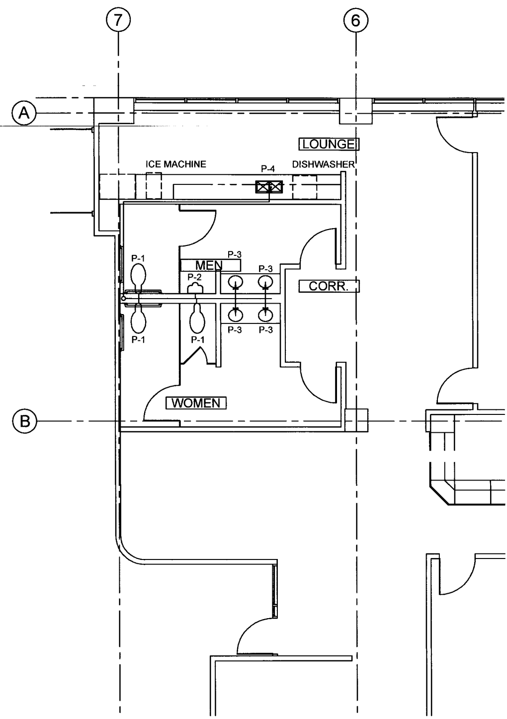
1 FIRST FLOOR PLUMBING PLAN Scale: 1/8" = 1'-0"
