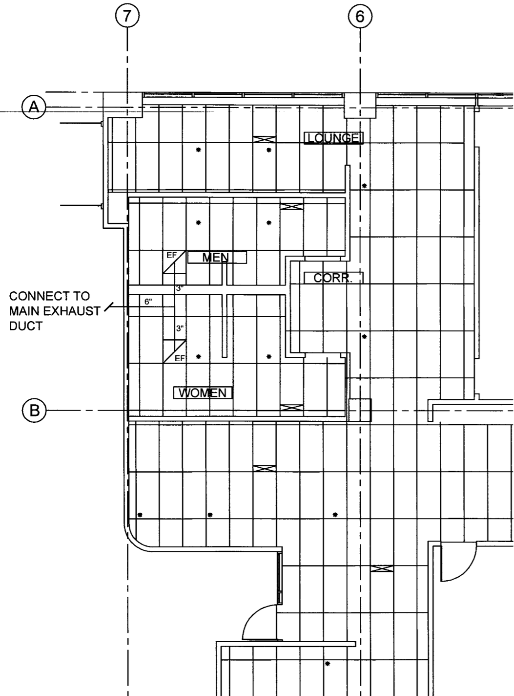
1 MECHANICAL PLAN Scale: 1/8" = 1'-0"
