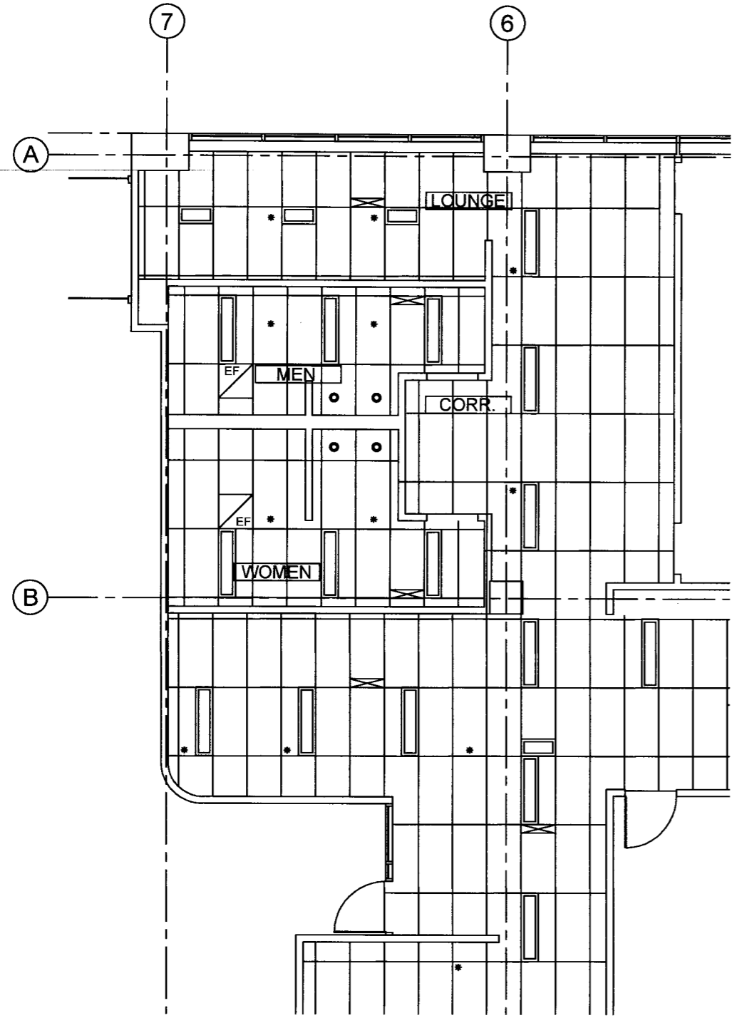
1 REFLECTED CEILING PLAN Scale: 1/8" = 1'-0"
