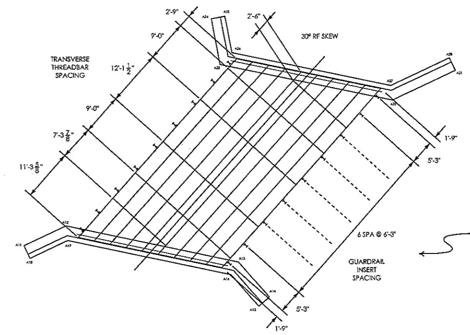
SUPERSTRUCTURE LAYOUT
