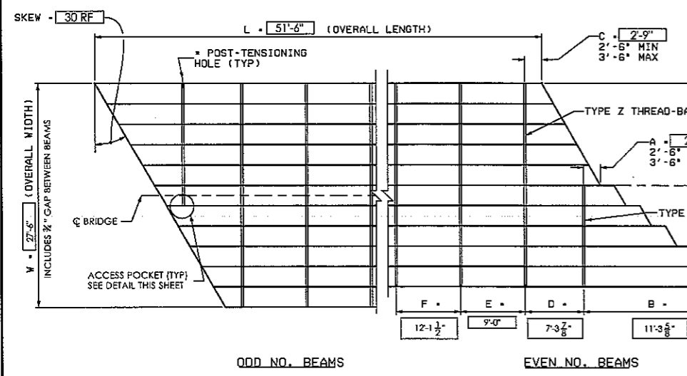
POST-TENSIONING BAR SPACING PLAN SKEW > 20°
