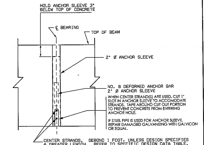
ANCHOR SLEEVE DETAIL
