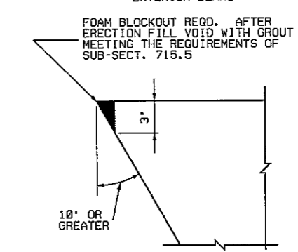
SKEW BLOCKOUT DETAIL
