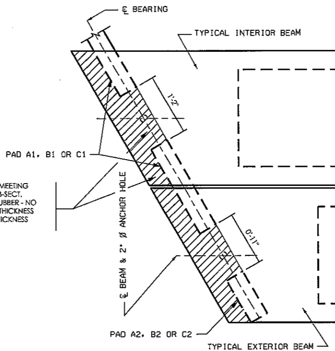
PLAN VIEW - BEARING PLACEMENT
