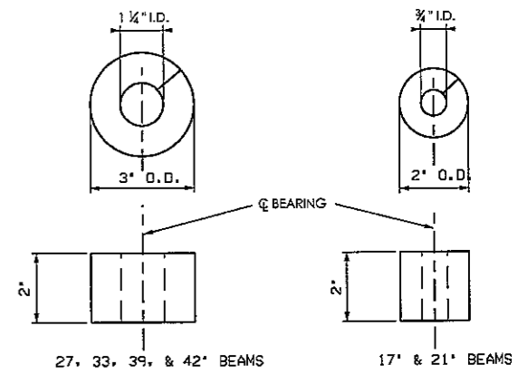
BLOCKOUT DETAILS
