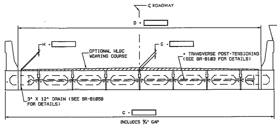
TYPICAL CROSS-SECTION WITH PARAPET OR CURB
