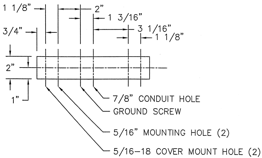
Mounting Bracket Detail
