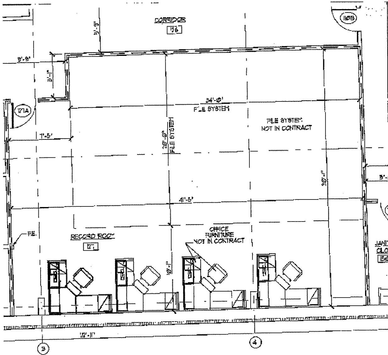
ENLARGED PROPOSED FLOOR PLAN - LEFT SIDE SCALE: 3/16" = 1'-0"
