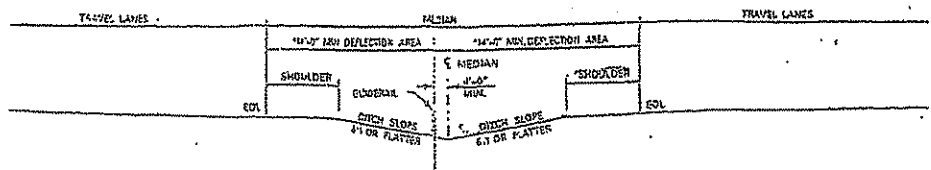
TYPICAL SECTION (DEFLECTION AREA ON MEDIAN SLOPES) DOUBLE FACE GUIDERAIL APPLICATION
