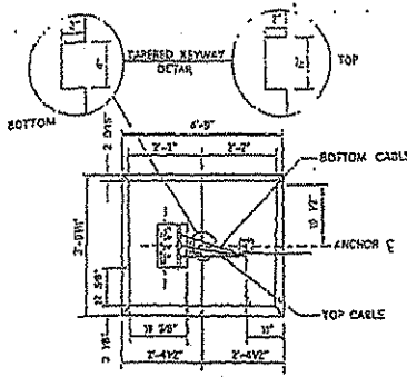
ANCHOR UNIT DETAIL TOP VIEW LEFT HAND (REINFORCEMENT NOT SHOWN) TWO PIECE
