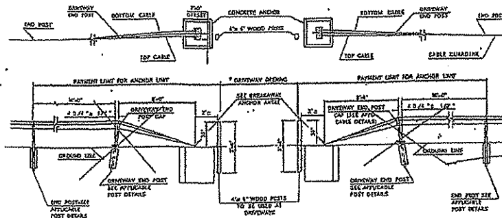
DRIVEWAYS AND OPENINGS (DOUBLE OR SINGLE FACE APPLICATION) *OPENINGS WILL BE PROVIDED ONLY FOR AREAS DESIGNATED ON ROADWAY PLAN SHEETS
