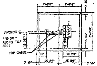
ANCHOR UNIT DETAIL TOP VIEW RIGHT HAND (REINFORCEMENT NOT SHOWN)
