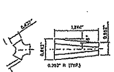
CABLE WEDGE TYPICAL WEDGE FOR ALL SPLICES AND CABLE FITTINGS
