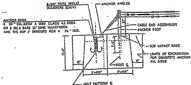
ANCHOR UNIT DETAIL LEFT HAND (REINFORCEMENT NOT SHOWN)
