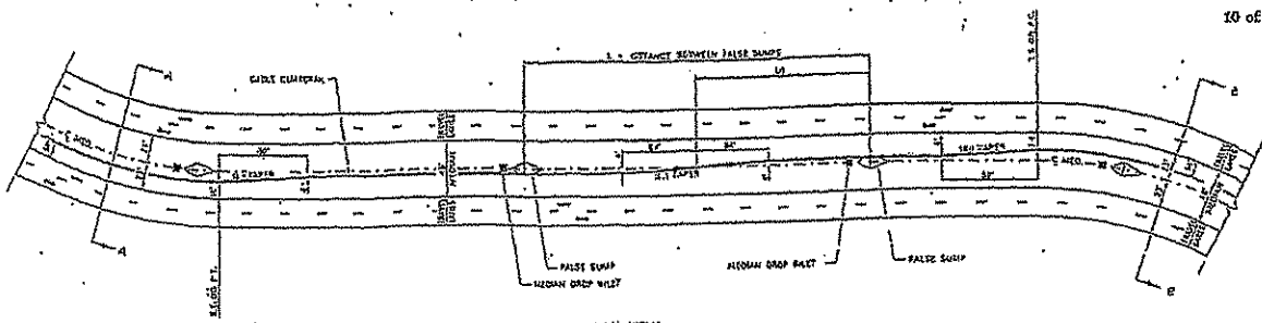
PLAN VIEW 46' MEDIAN CABLE GUARDRAIL TRANSITIONS WITH SUPERELEVATION AND/OR FALSE BUMPS
