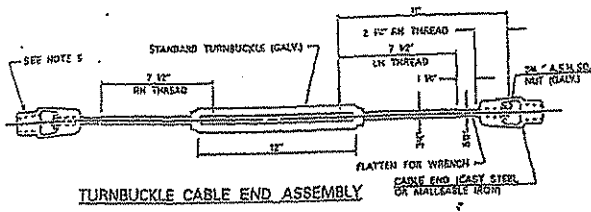
SPRING CABLE END ASSEMBLY (COMPENSATING DEVICE)
