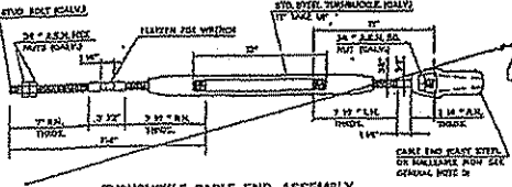
TURNBUCKLE CABLE END ASSEMBLY
