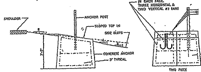
ANCHOR UNIT & RE-BAR INSTALLATION DETAIL
