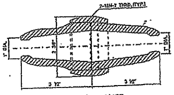
CABLE SPLICE NOTE: USE WITH WEDGE
