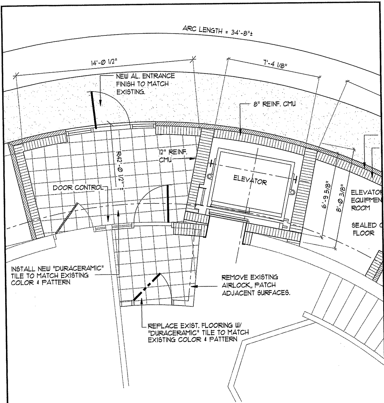
FLOOR TILE CHANGES IN LOWER INTERIOR LOBBY
