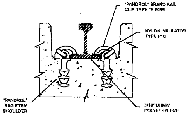
RAIL DETAIL
