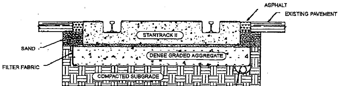
INSTALLATION SECTION
