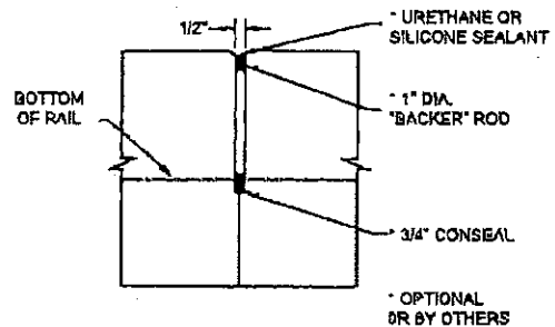
CONNECTION DETAIL
