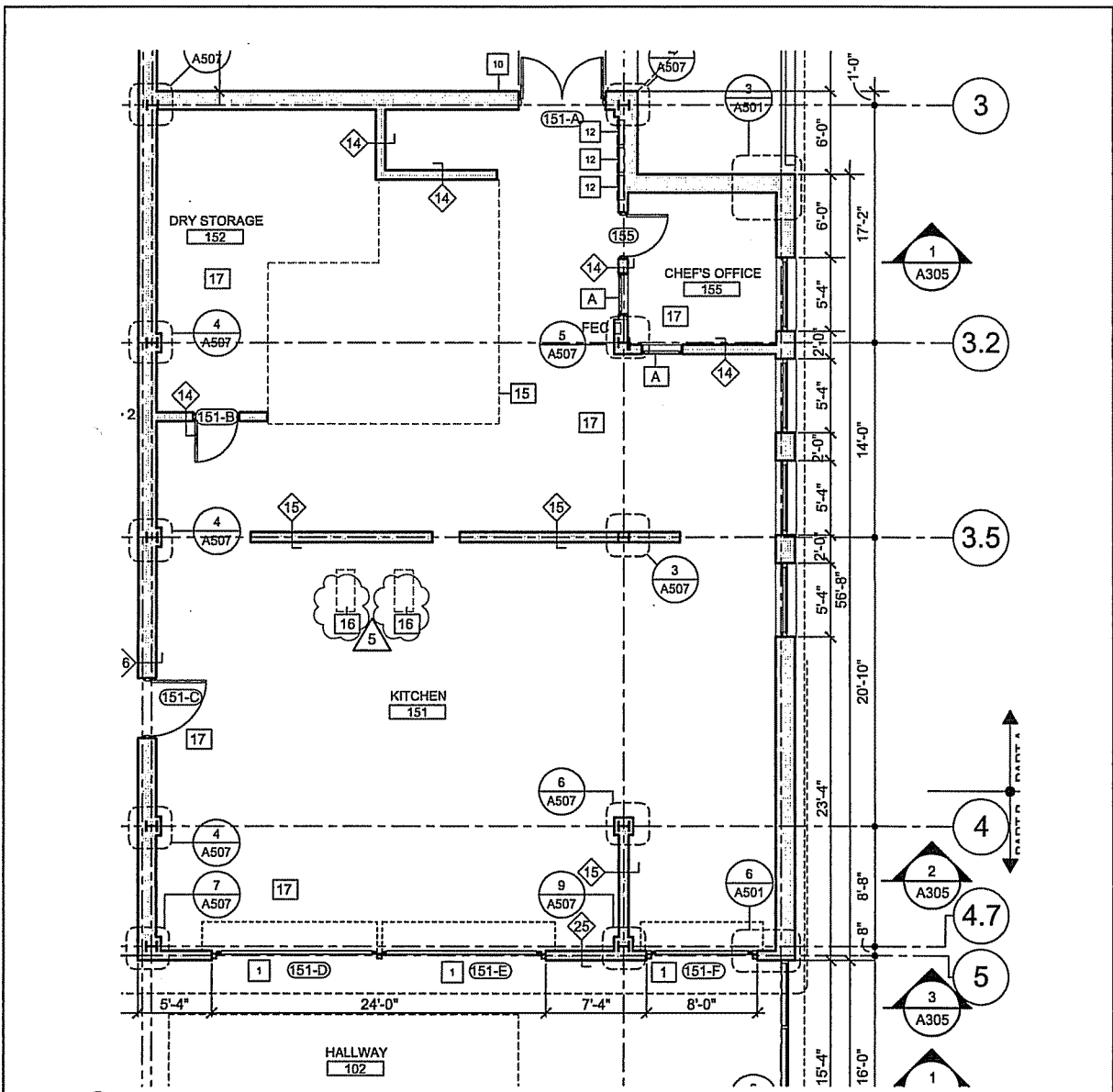
1 FIRST FLOOR PLAN - PART A 1/8" = 1'-0"
