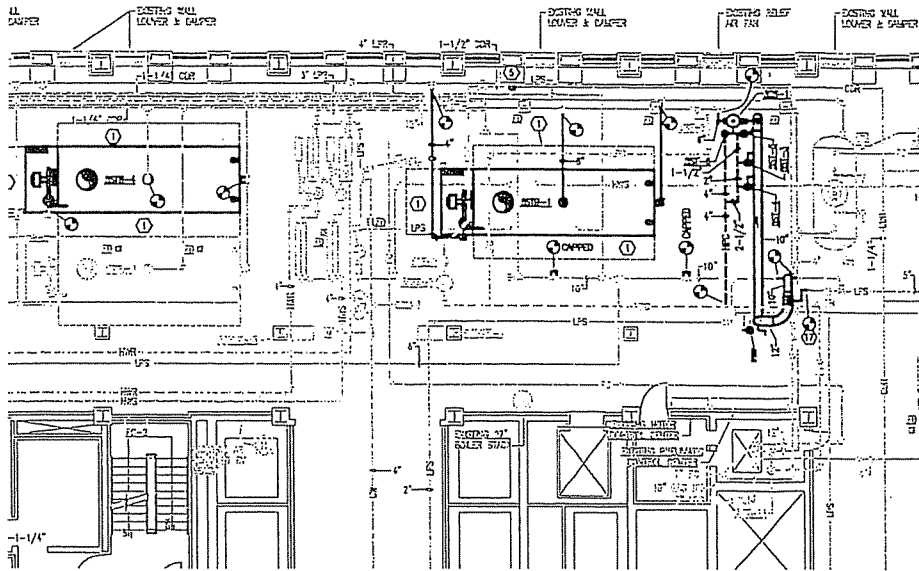
BUILDING #5-(FUTURE BOILER EXPANSION)-NEW
