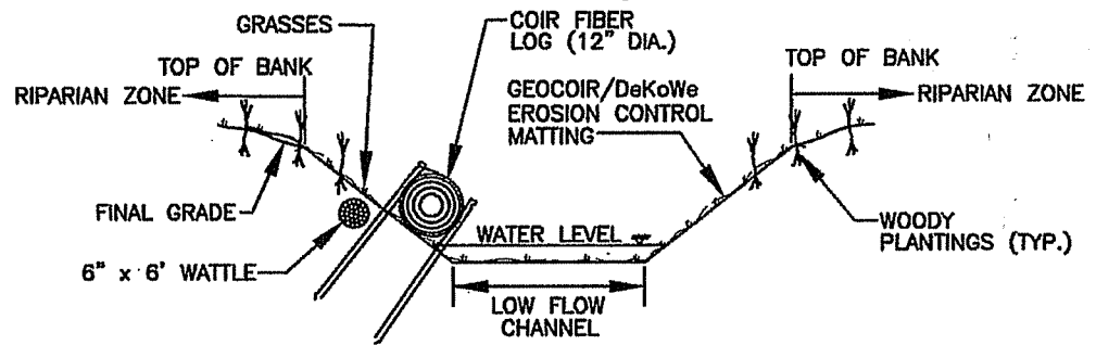
SECTION (2/A12)
