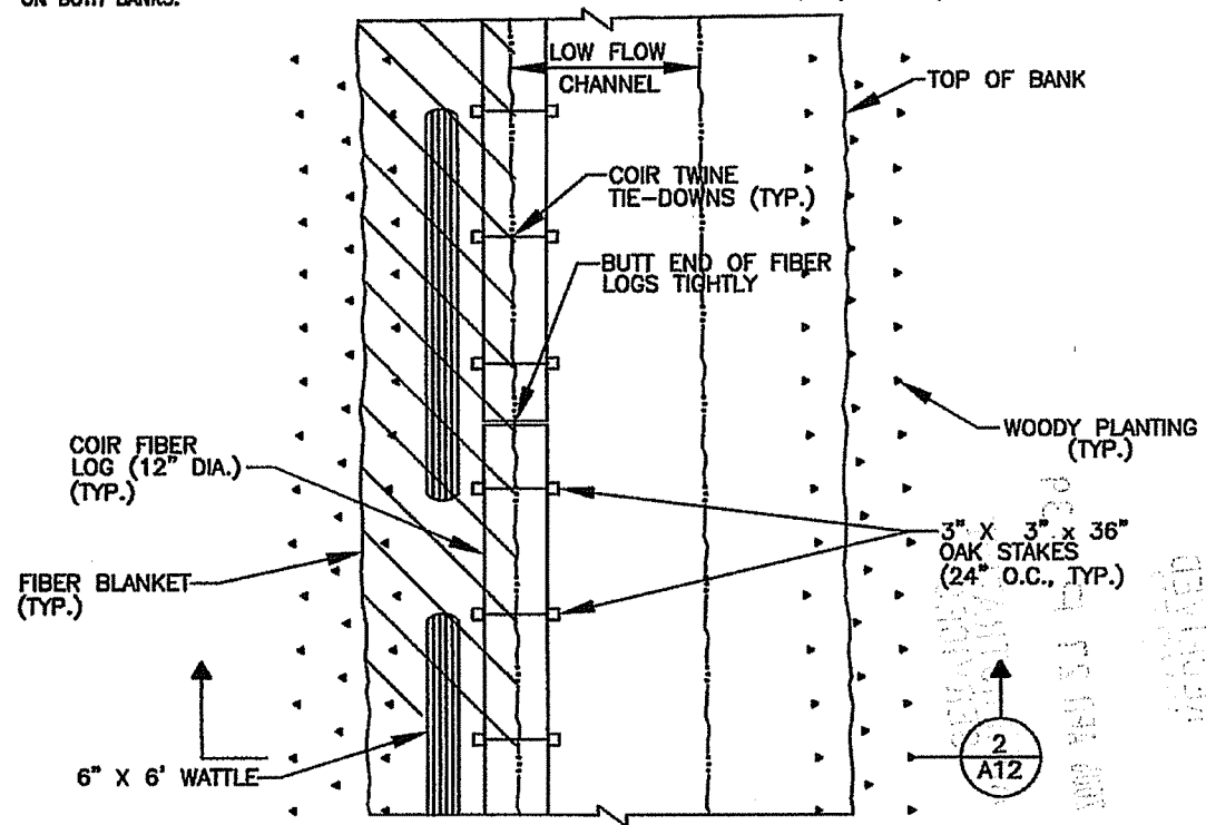
PLAN (1/A12)
