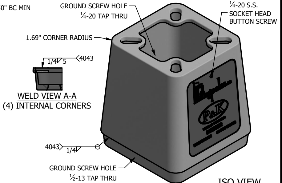
ISO VIEW
